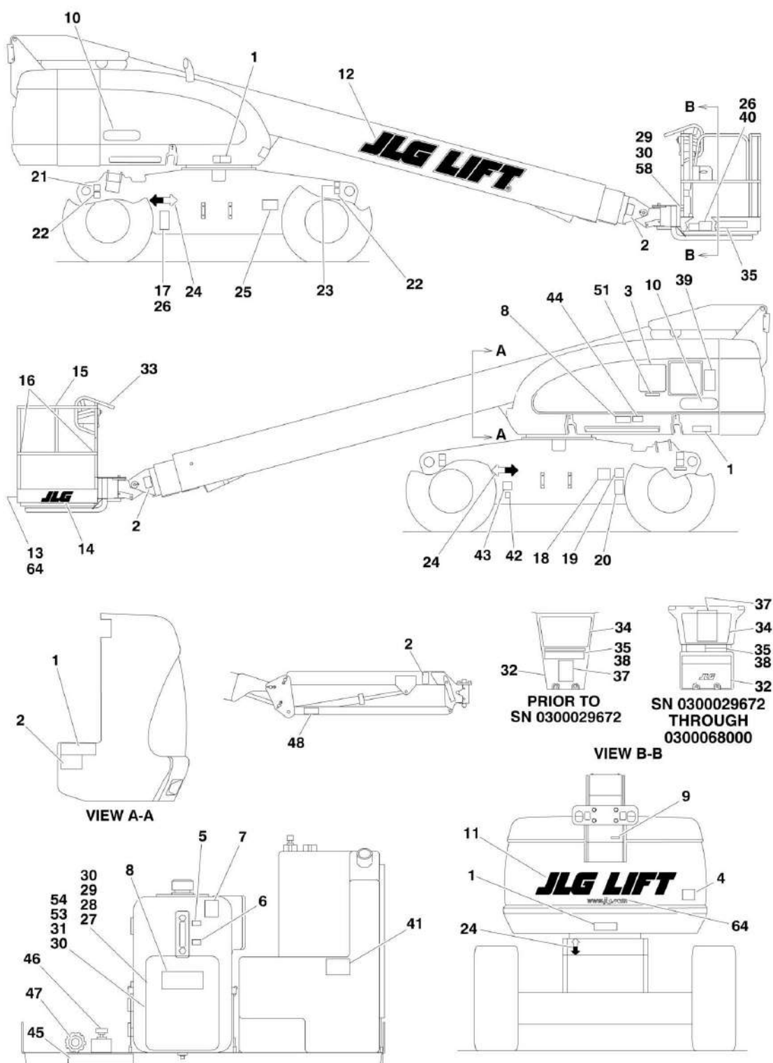
FIGURE 8-2. DECAL INSTALLATION - COUNTRY SPEC
