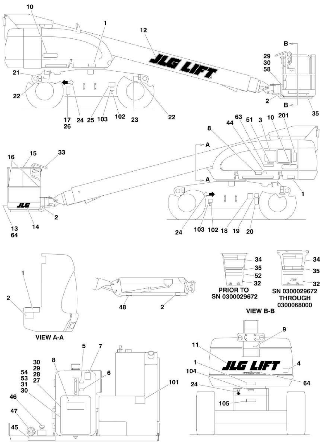
FIGURE 8-1. DECALS INSTALLATION - STANDARD
