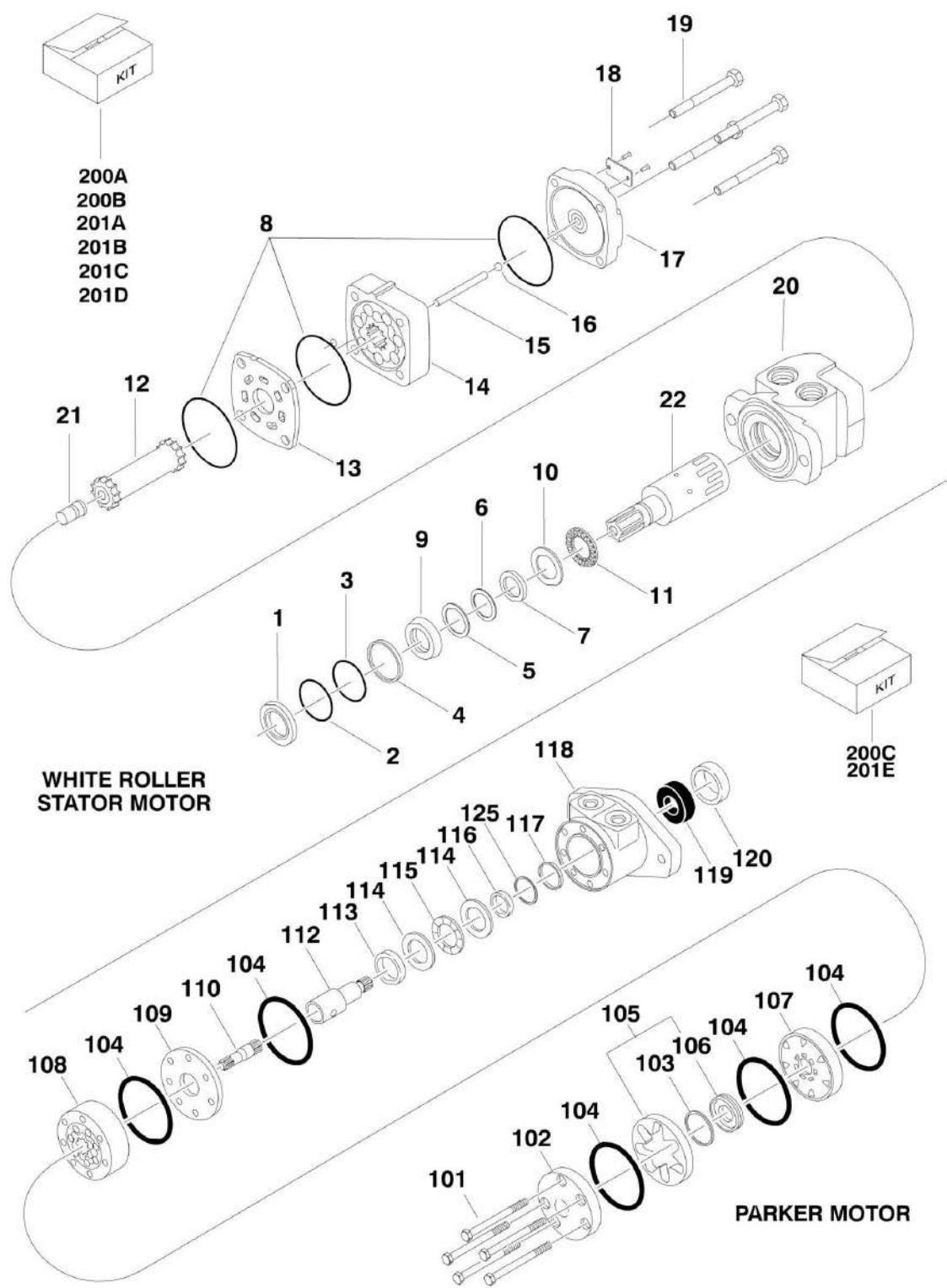
FIGURE 2-7. SWING MOTOR ASSEMBLIES
