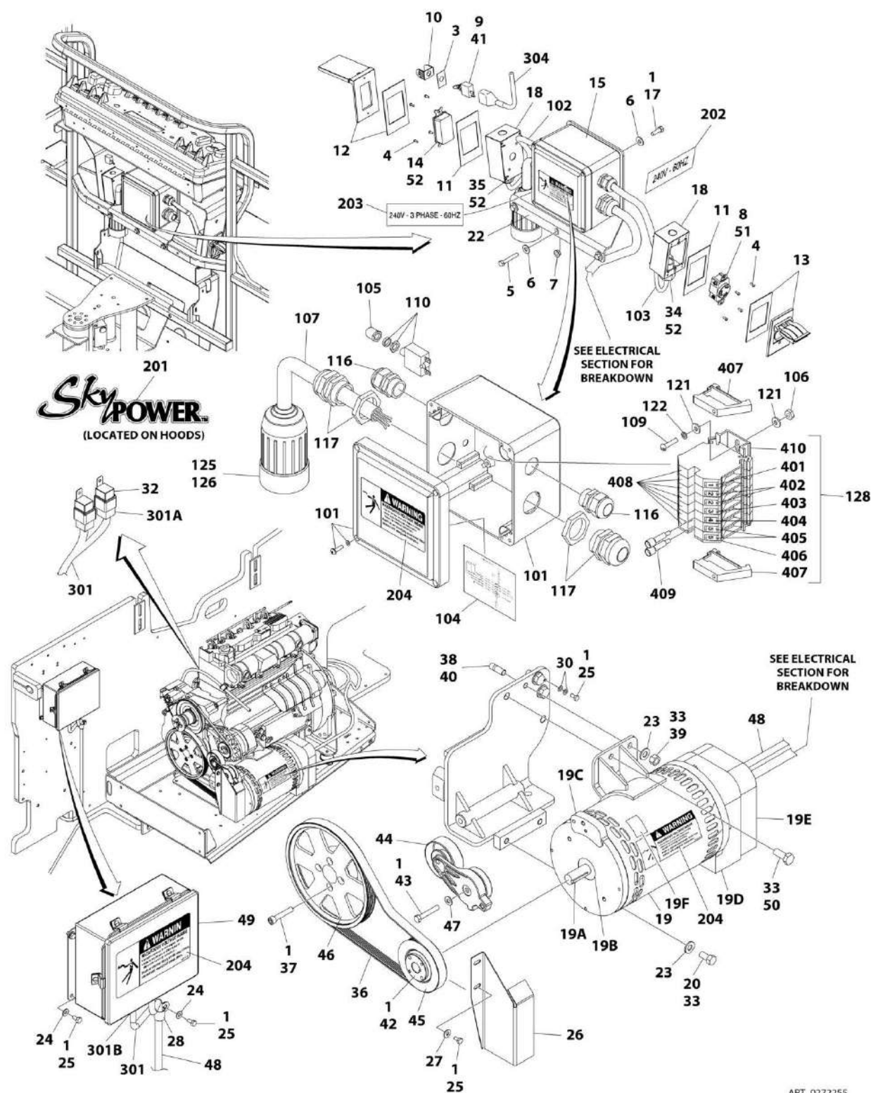
FIGURE 2-13. 7500W SKYPOWER GENERATOR INSTALLATION - DEUTZ MACHINES (ANSI AND CSA SPECS)
