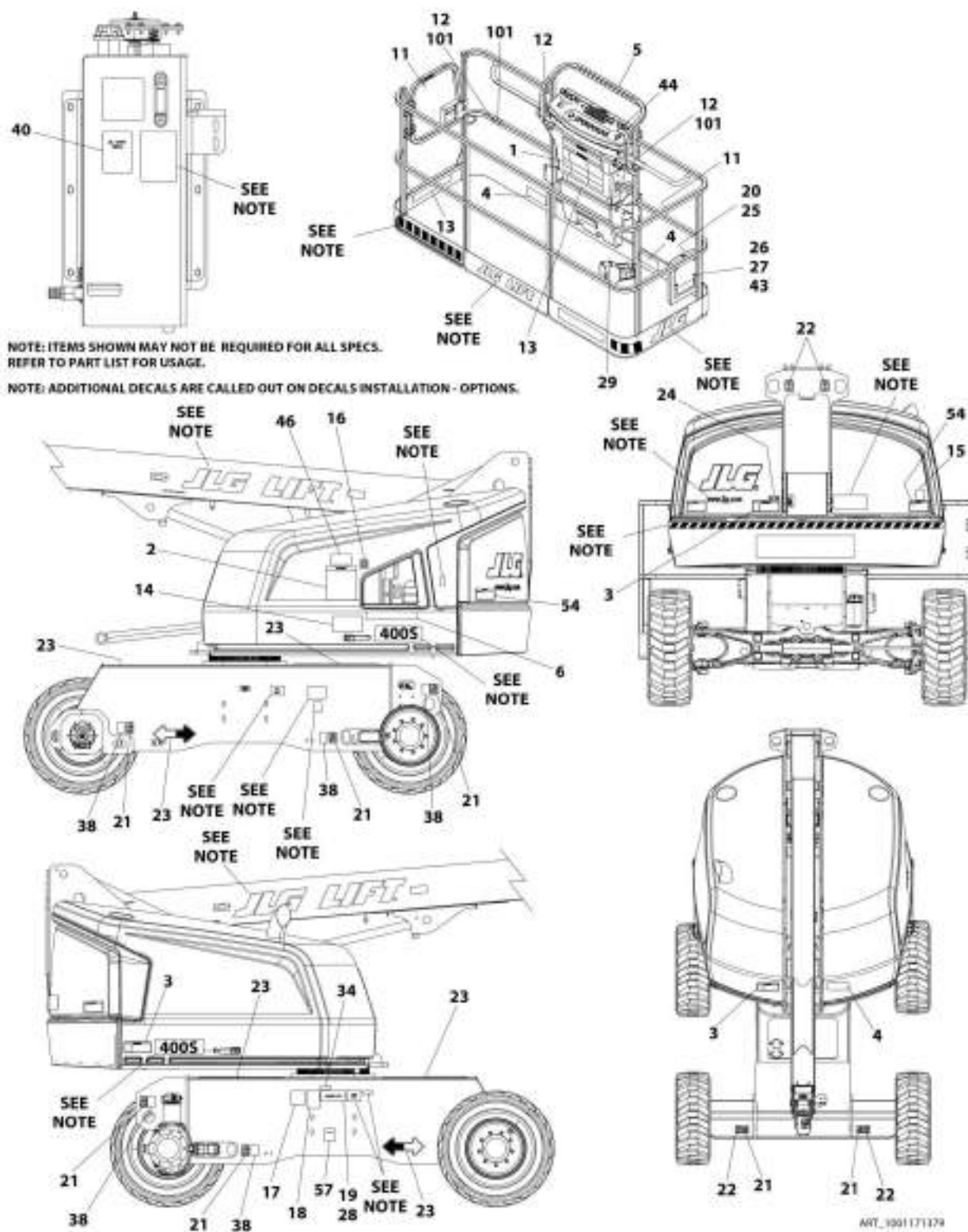
FIGURE 9-11. DECAL INSTALLATION - CHINESE SPEC (DUAL LANGUAGE - ENGLISH/CHINESE) (460SJ)
