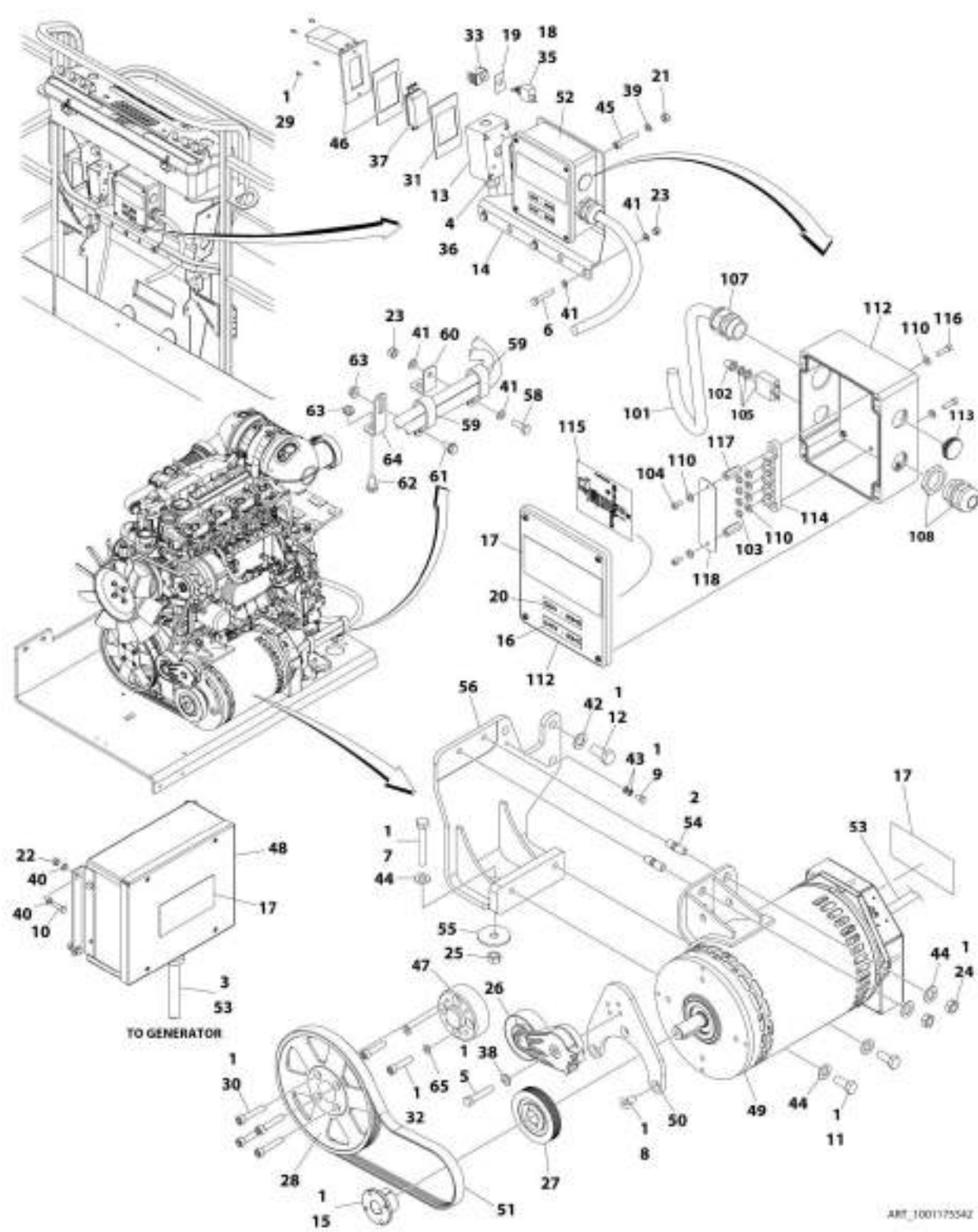
FIGURE 3-64. GENERATOR INSTALLATION - 4000W/60HZ (DEUTZ D2.9L4 ENGINE)
