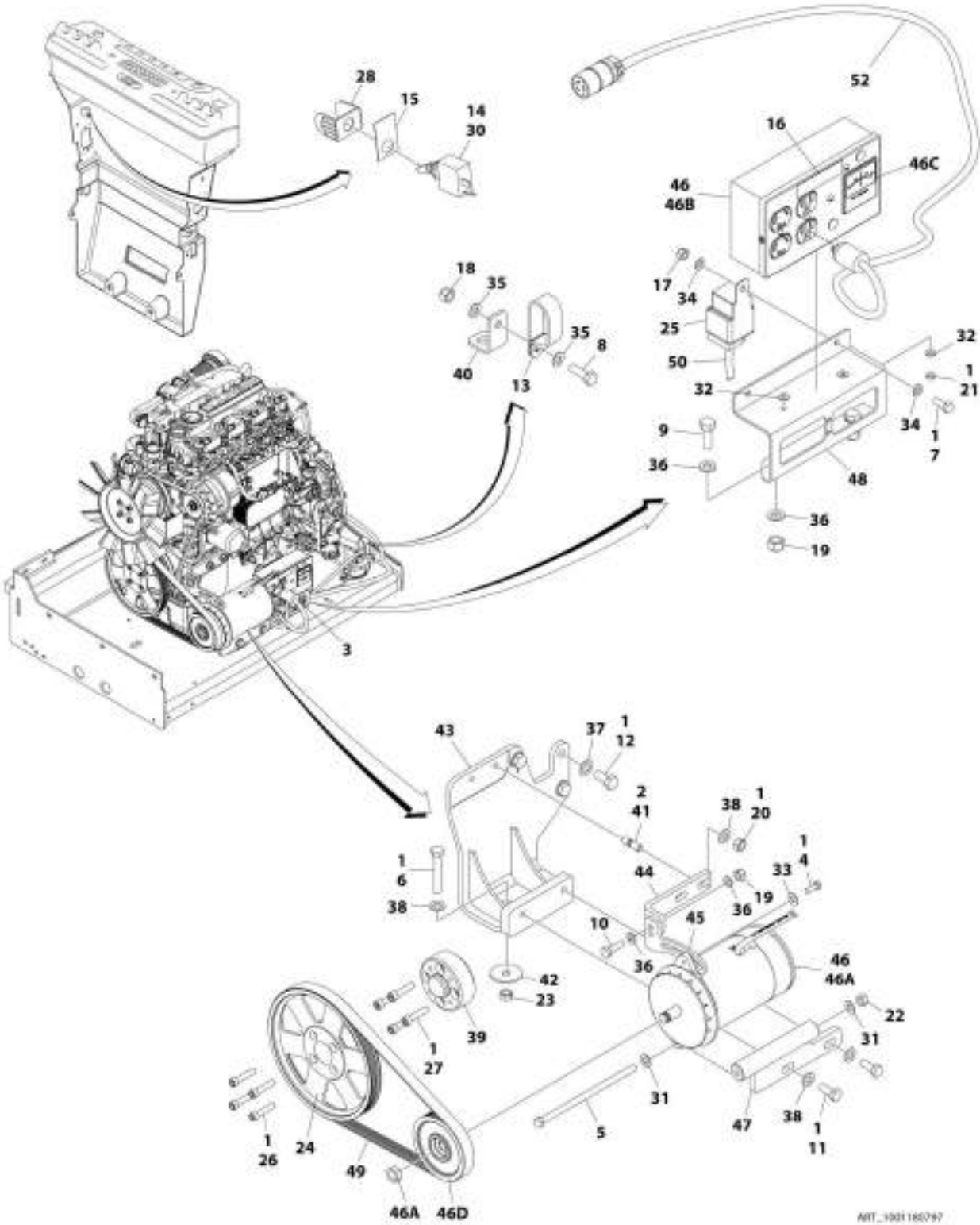
FIGURE 3-59. GENERATOR INSTALLATION - 2500W/60HZ (DEUTZ D2.9L4 ENGINE)
