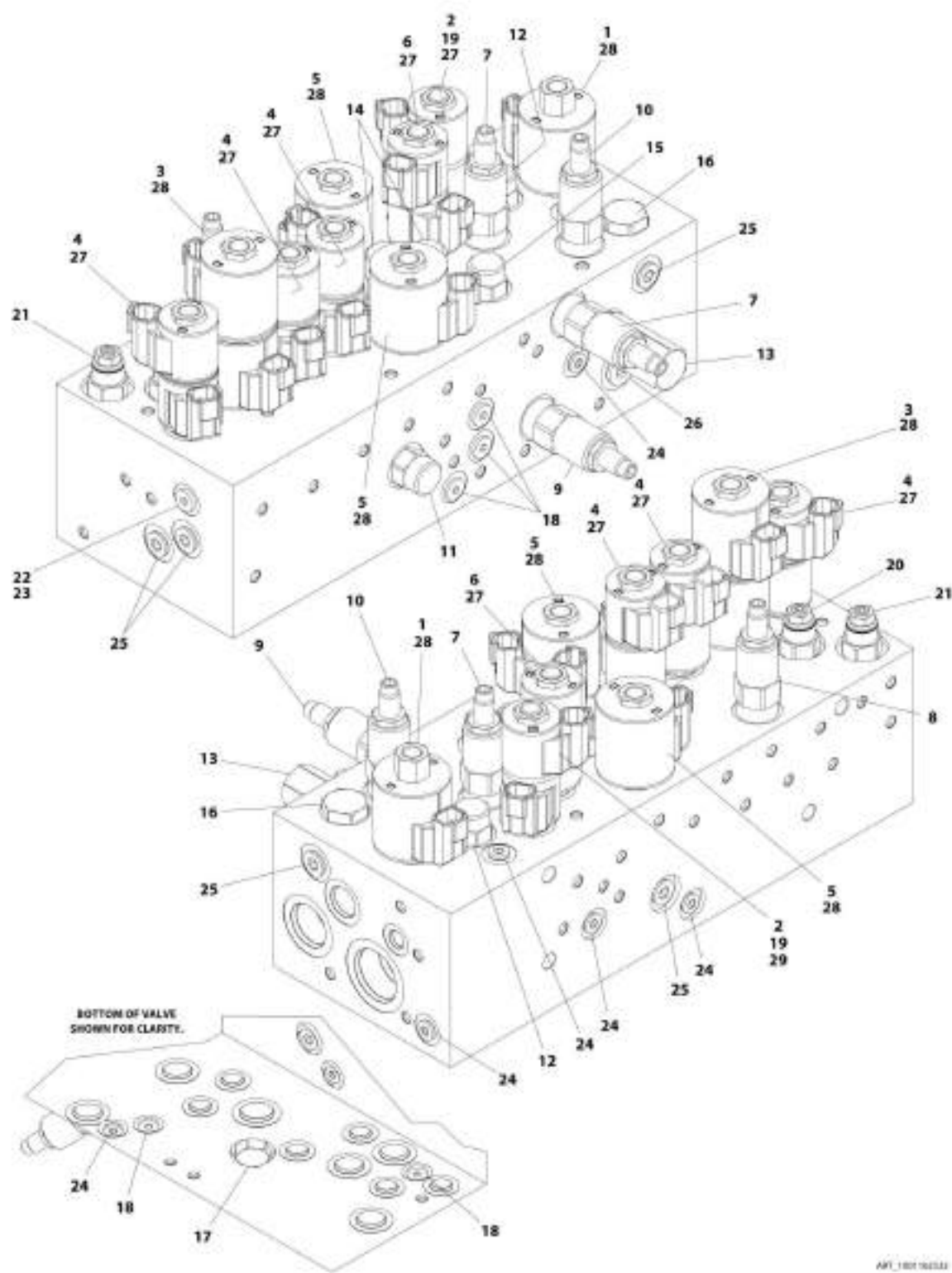
FIGURE 2-4. MAIN VALVE ASSEMBLY - 460SJ
