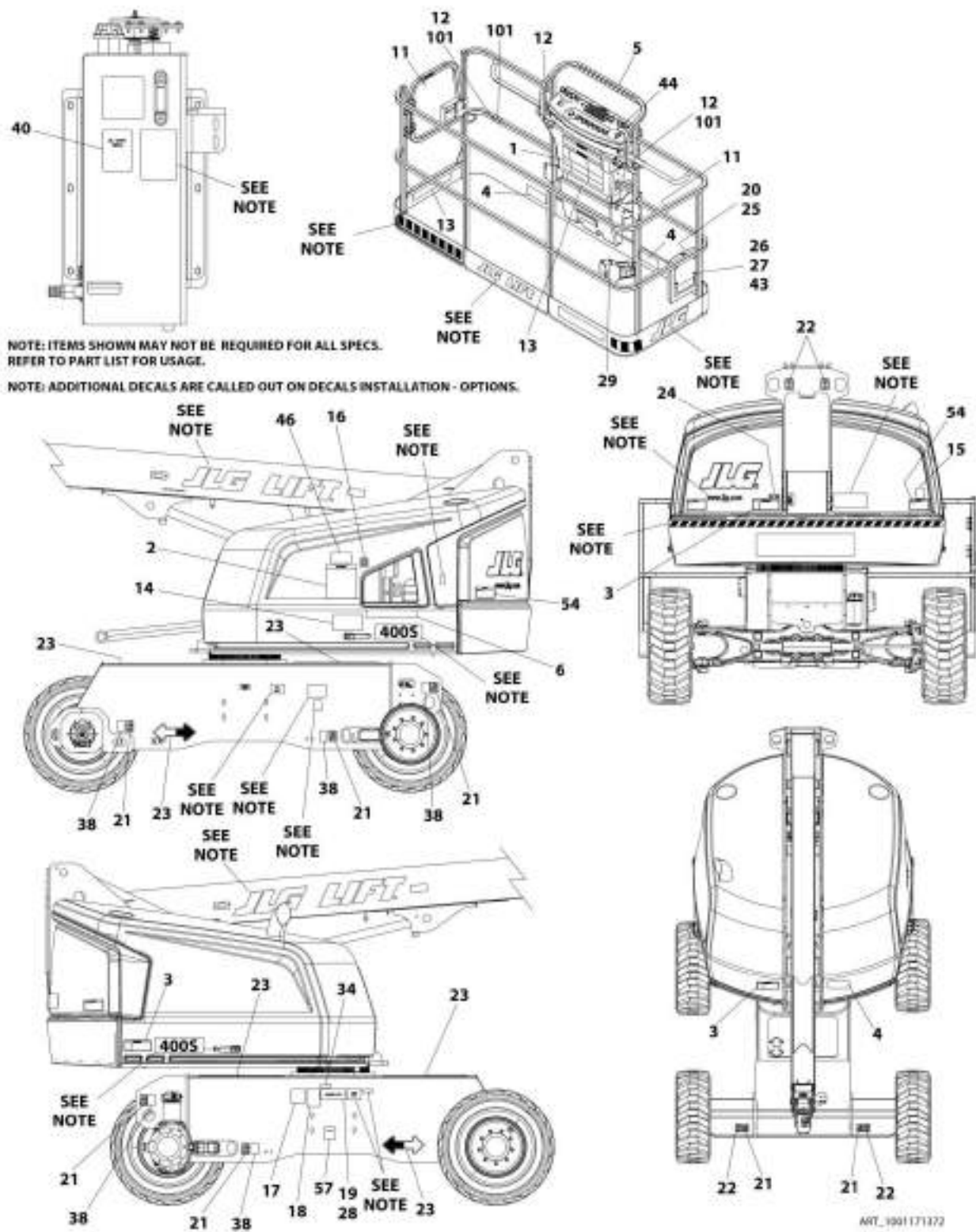
FIGURE 9-18. DECAL INSTALLATION - KOREAN SPEC (DUAL LANGUAGE - ENGLISH/KOREAN) (400S)
