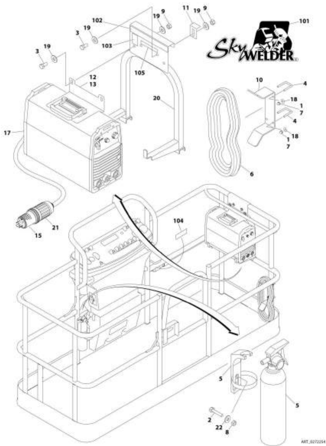
FIGURE 5-35. SKYWELDER INSTALLATION (60HZ)
