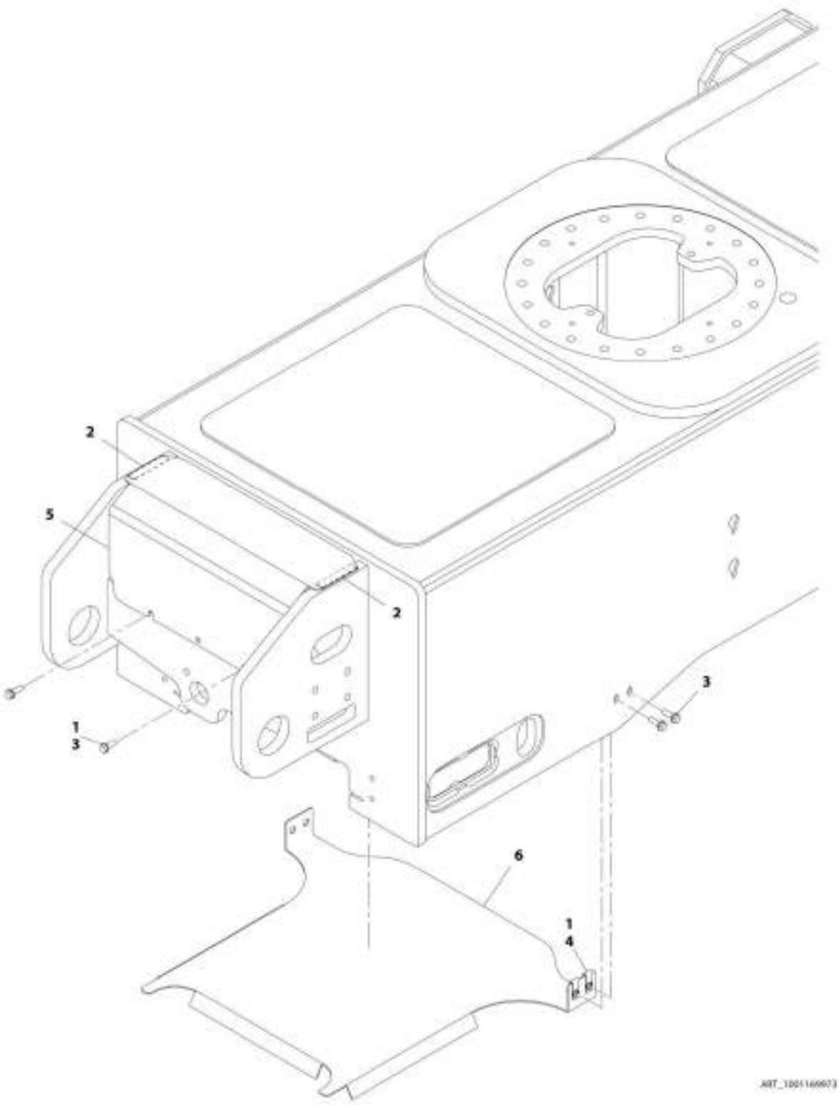
FIGURE 1-20. FRAME SHIELD INSTALLATION - WITHOUT TOW BAR
