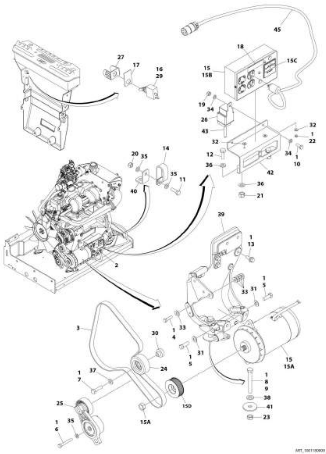
FIGURE 3-60. GENERATOR INSTALLATION - 2500W/60HZ (GM ENGINE)
