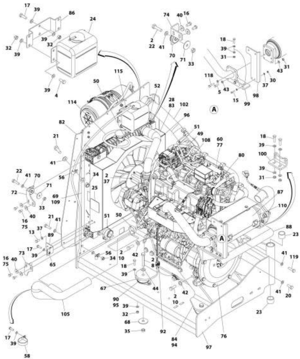
FIGURE 3-46. ENGINE ASSEMBLY - KUBOTA ENGINE (WITH ARCTIC PACKAGE) (SN 0300241778 to Present)
