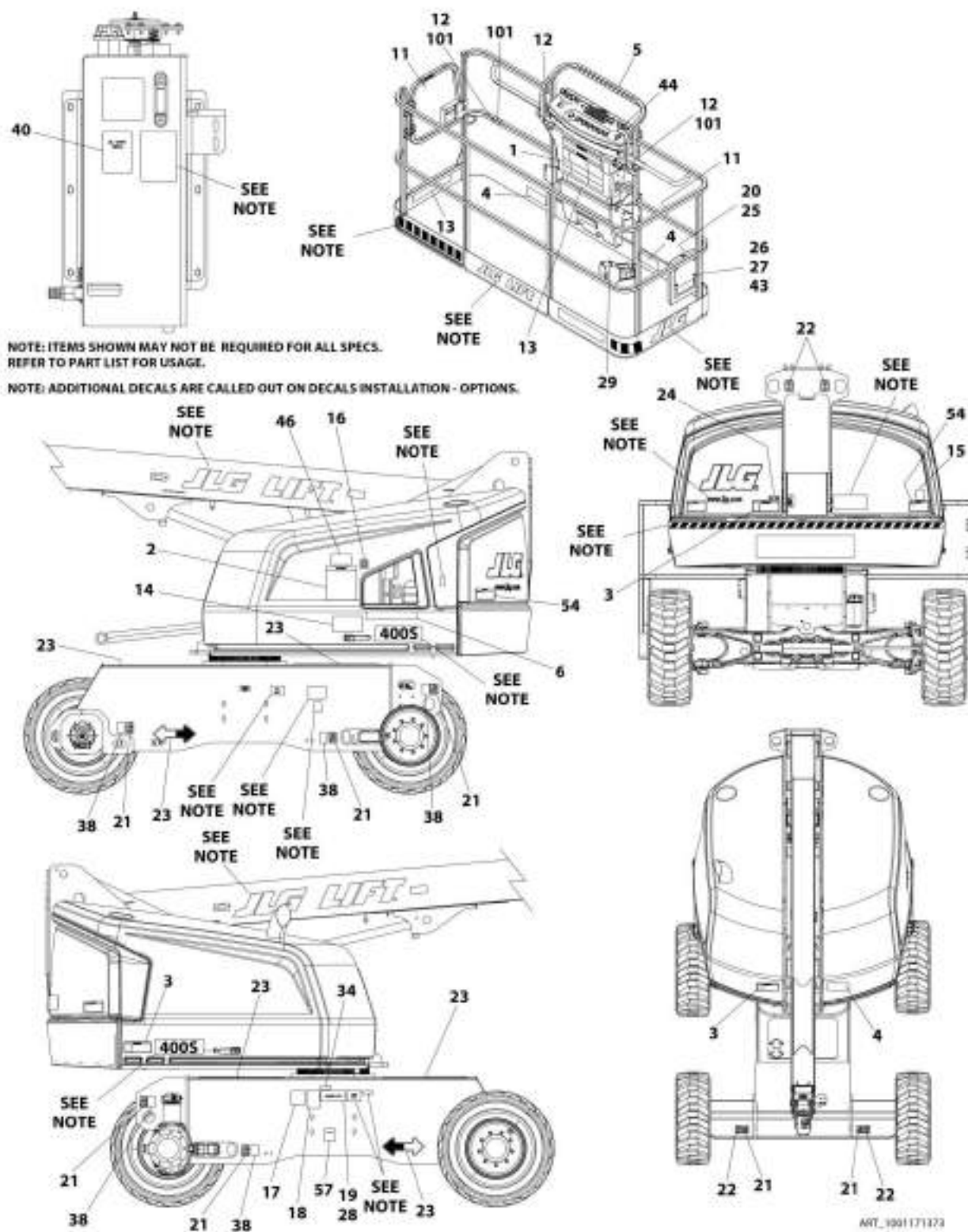
FIGURE 9-19. DECAL INSTALLATION - KOREAN SPEC (DUAL LANGUAGE - ENGLISH/KOREAN) (460SJ)
