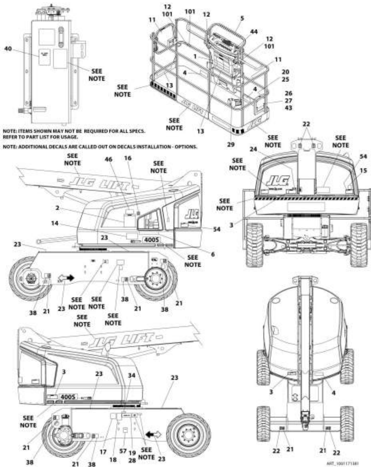
FIGURE 9-9. DECAL INSTALLATION - BRAZIL SPEC (DUAL LANGUAGE - PORTUGUESE/SPANISH) (460SJ)
