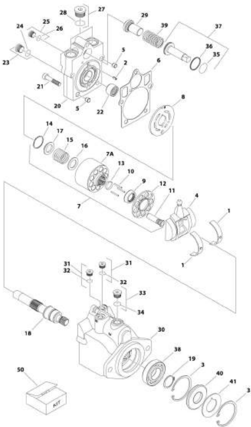
FIGURE 1-9. DRIVE MOTOR ASSEMBLY (2WD)
