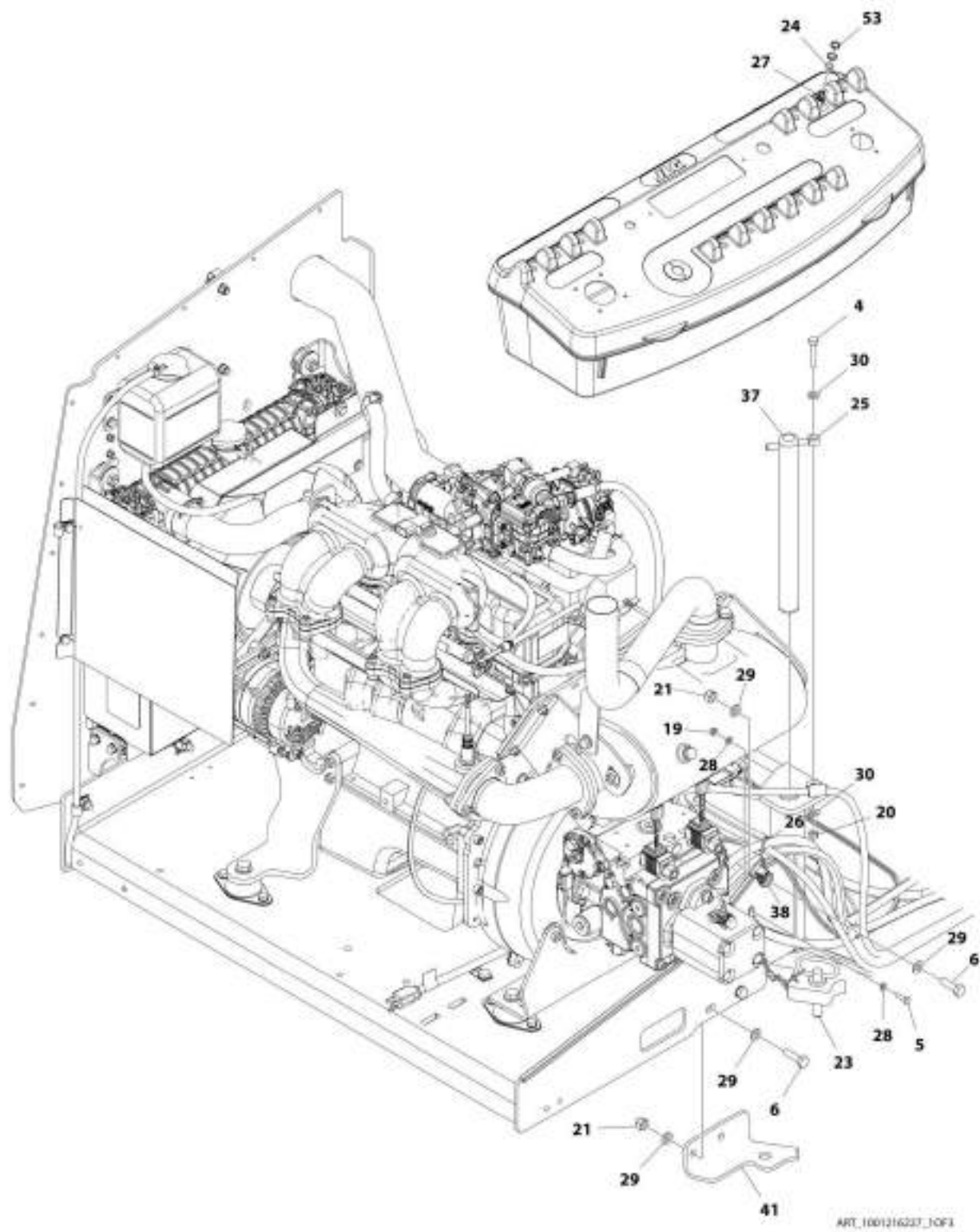
FIGURE 3-28. ENGINE INSTALLATION - GM ENGINE (WITH ARCTIC PACKAGE) (SN 0300222292 to Present)
