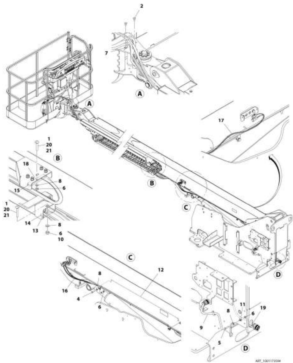
FIGURE 4-19. CABLES AND CLAMPS INSTALLATION - 400S (ANSI, ANSI EXPORT, CSA AND CHINA SPECS)
