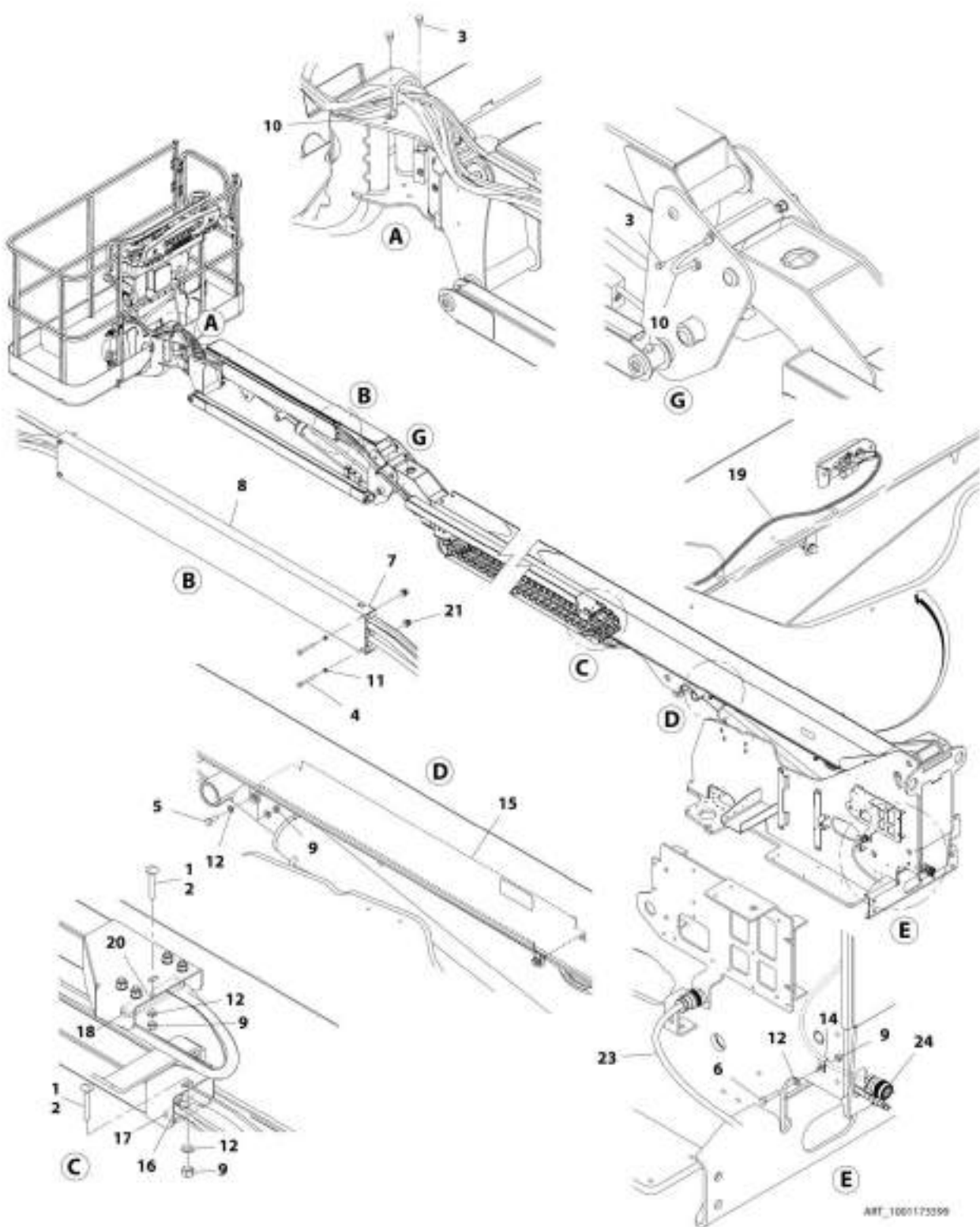
FIGURE 4-24. CABLES AND CLAMPS INSTALLATION - 460SJ (ALL SPECS) (SN 0300212083 to Present, SN E300000100 to Present, SN 1300007289 through 1300007393)
