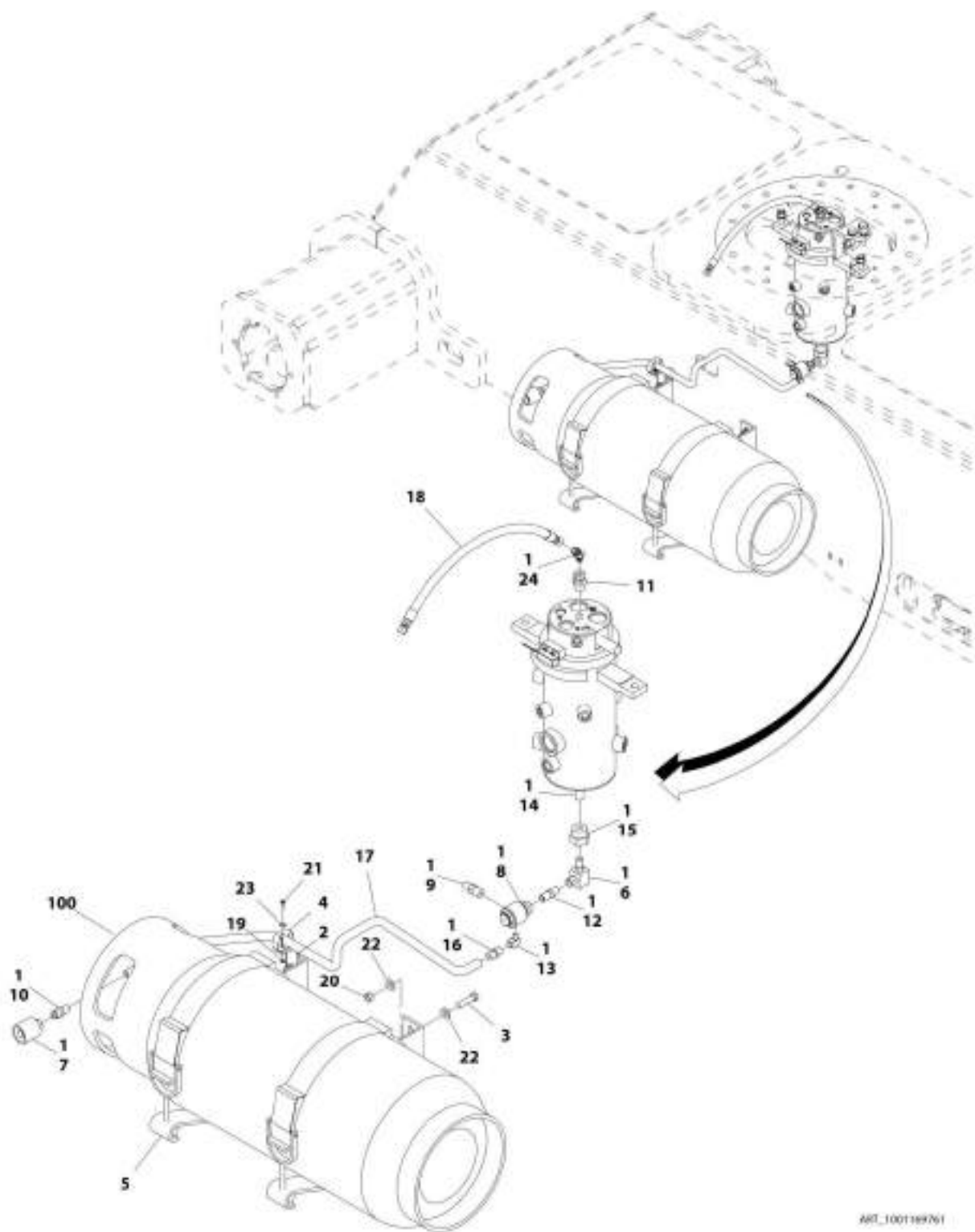
FIGURE 1-24. LP TANK BRACKETS INSTALLATION
