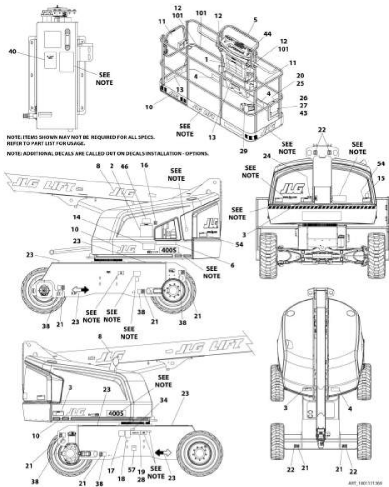
FIGURE 9-6. DECAL INSTALLATION - CE SPEC (400S)
