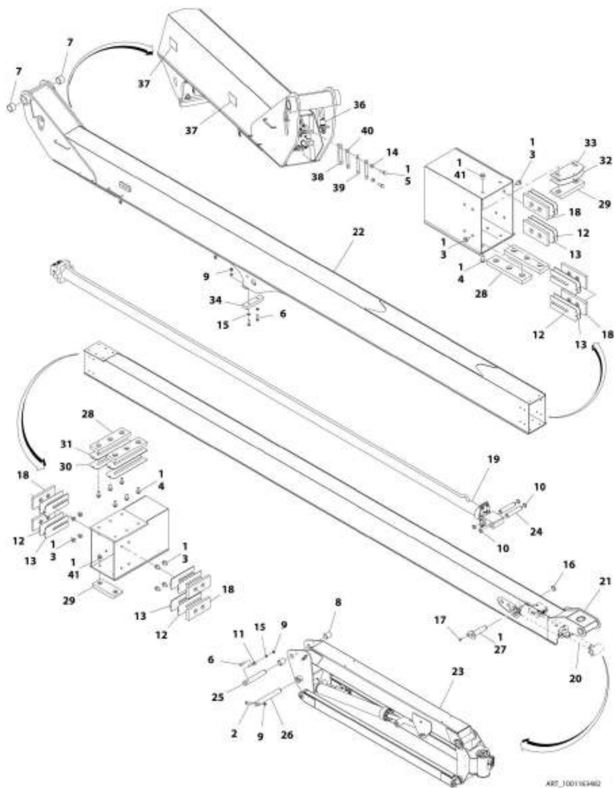
FIGURE 4-5. MAIN BOOM ASSEMBLY - 460SJ (SN 0300203771 to Present, SN E300000100 through E300004333)
