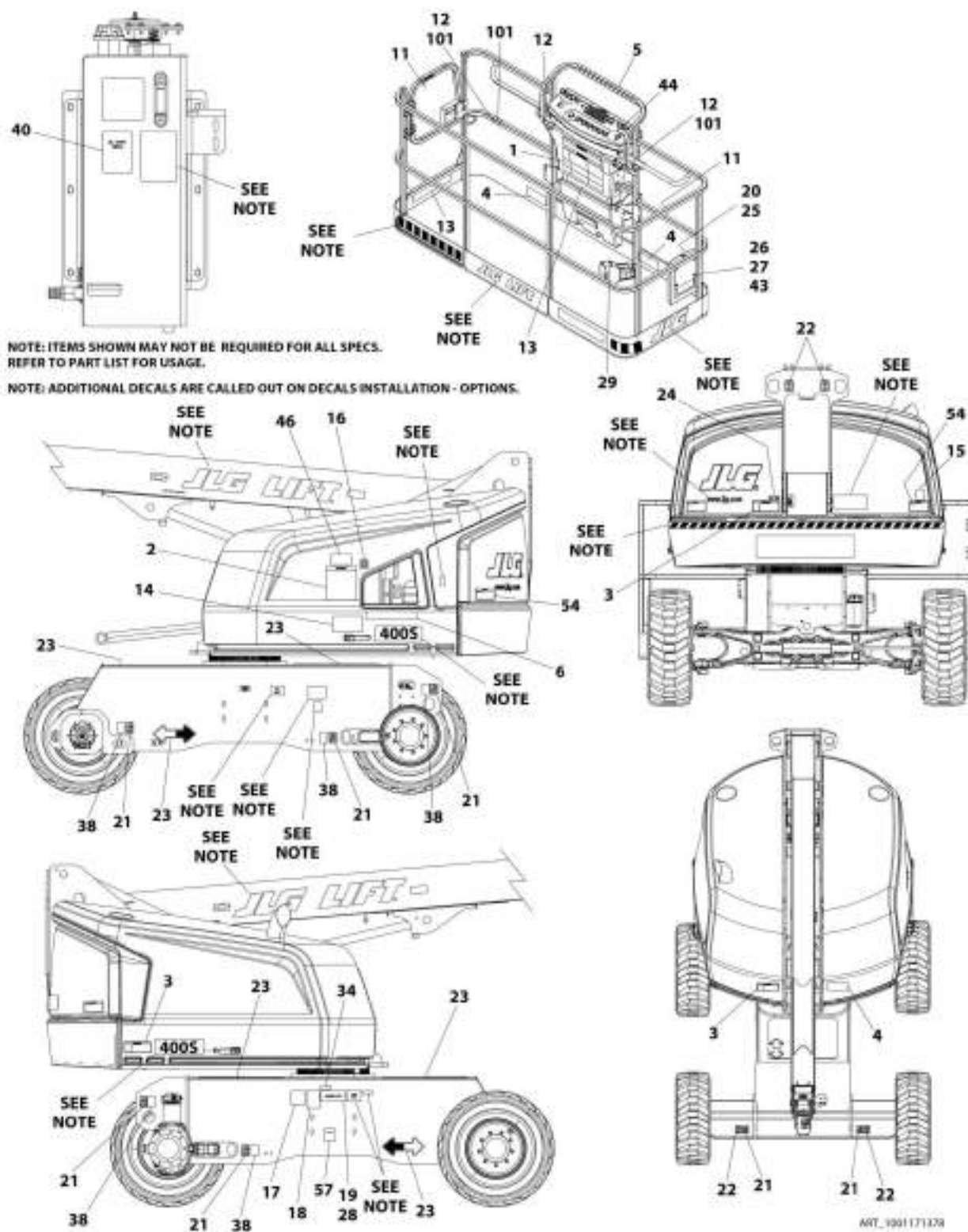
FIGURE 9-10. DECAL INSTALLATION - CHINESE SPEC (DUAL LANGUAGE - ENGLISH/CHINESE) (400S)
