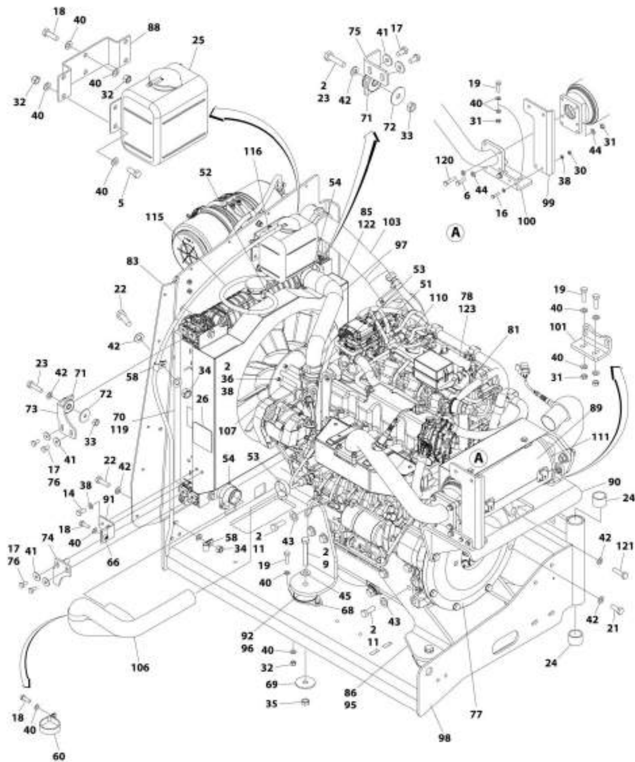
FIGURE 3-38. ENGINE ASSEMBLY - KUBOTA ENGINE (WITHOUT ARCTIC PACKAGE) (SN 0300203771 through 0300241777)
