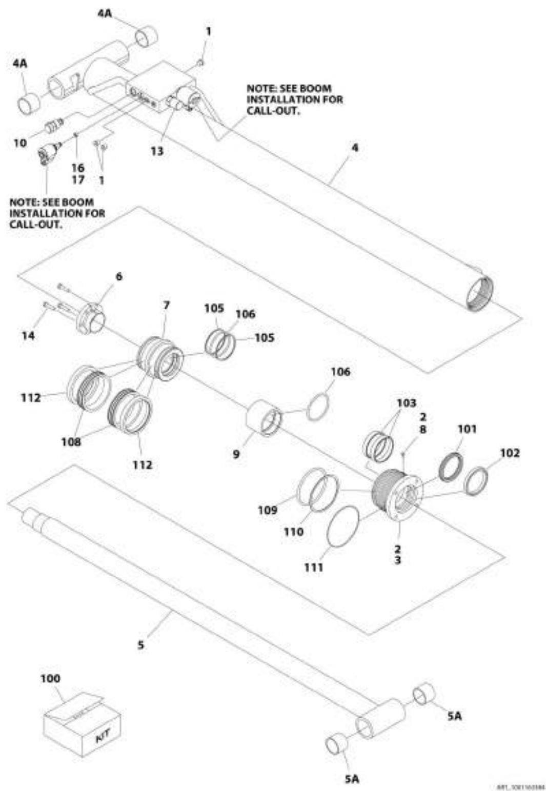
FIGURE 6-3. LIFT CYLINDER ASSEMBLY - MAIN BOOM (SN 0300203771 through 0300204034)
