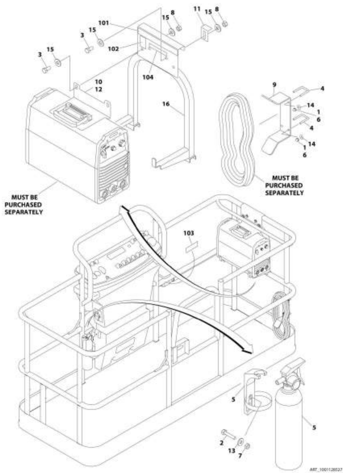
FIGURE 5-36. SKYWELDER PREP PACKAGE (60HZ)
