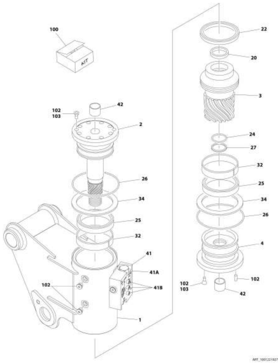
FIGURE 4-10. ROTATOR ASSEMBLY - 400S (SN 0300244183 to Present, SN E300005674 to Present)
