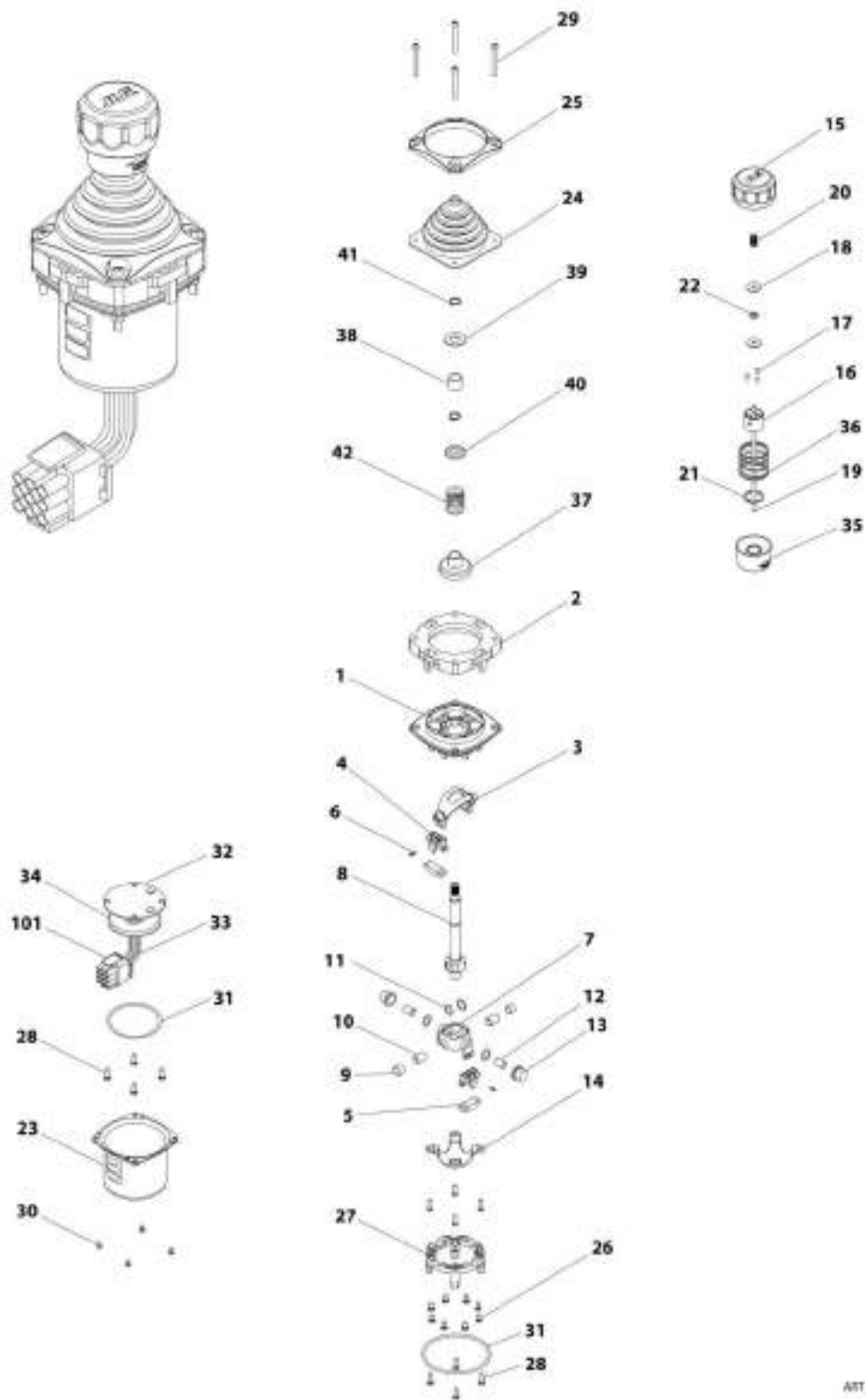
FIGURE 5-24. CONTROLLER ASSEMBLY - LIFT AND SWING
