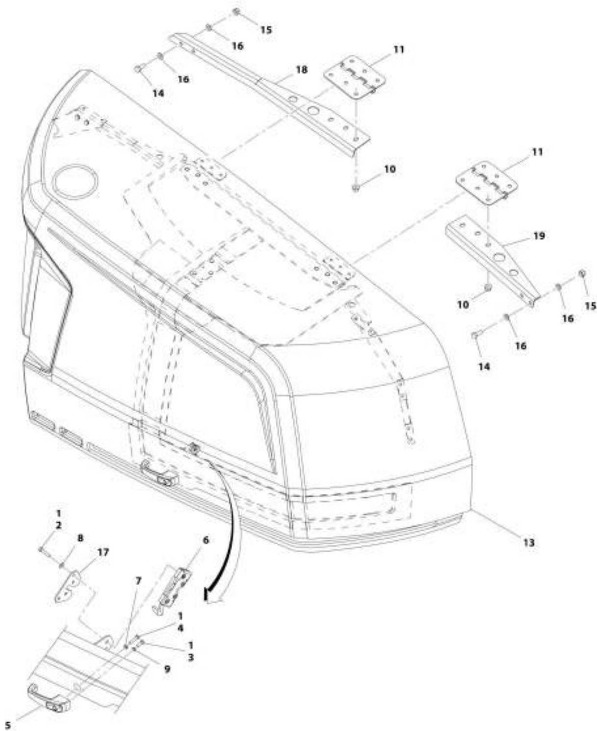
FIGURE 2-38. ABS HOOD ASSEMBLY - ENGINE SIDE
