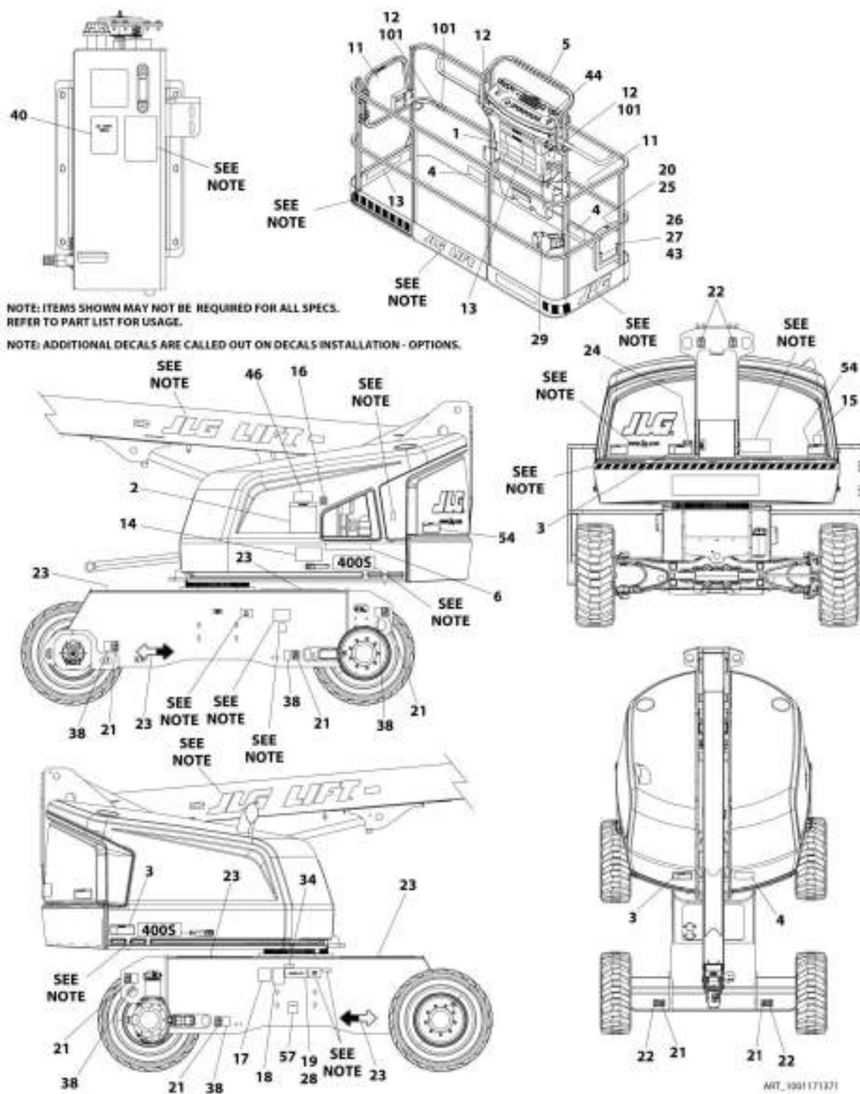
FIGURE 9-17. DECAL INSTALLATION - JAPANESE SPEC (DUAL LANGUAGE - ENGLISH/JAPANESE) (460SJ)
