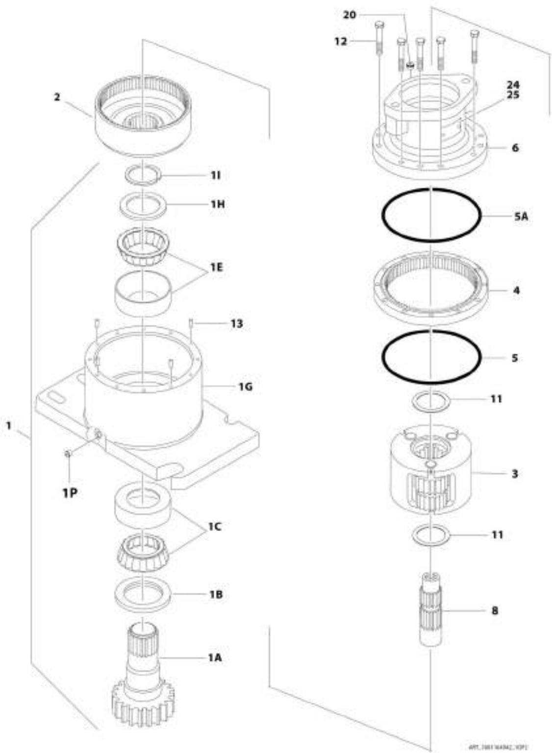
FIGURE 2-8. SWING HUB/MOTOR ASSEMBLY (Prior to SN 0300249769, Prior to SN E300006129)
