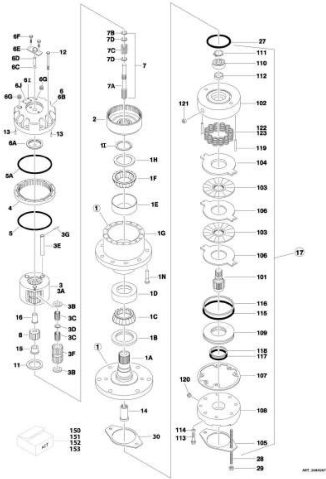
FIGURE 1-6. DRIVE HUB AND BRAKE ASSEMBLY - REAR
