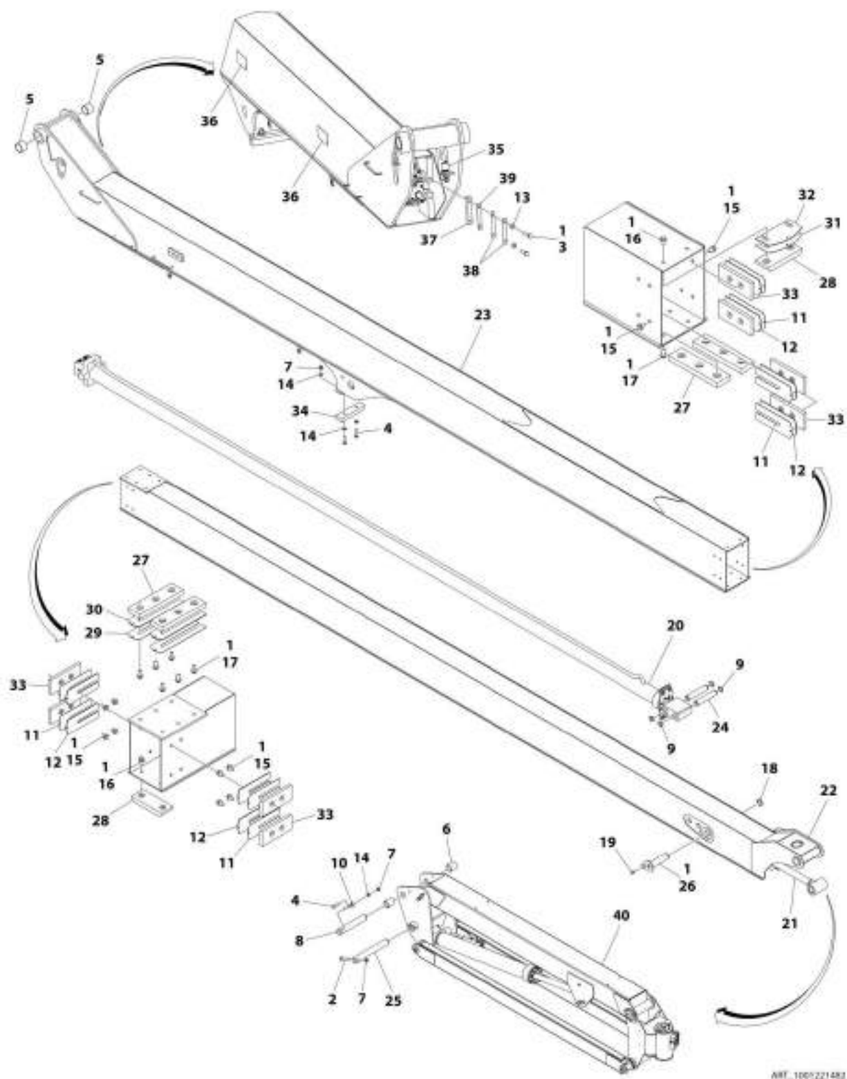
FIGURE 4-6. MAIN BOOM ASSEMBLY - 460SJ (SN E300004334 to Present, SN 1300007289 through 1300007393)
