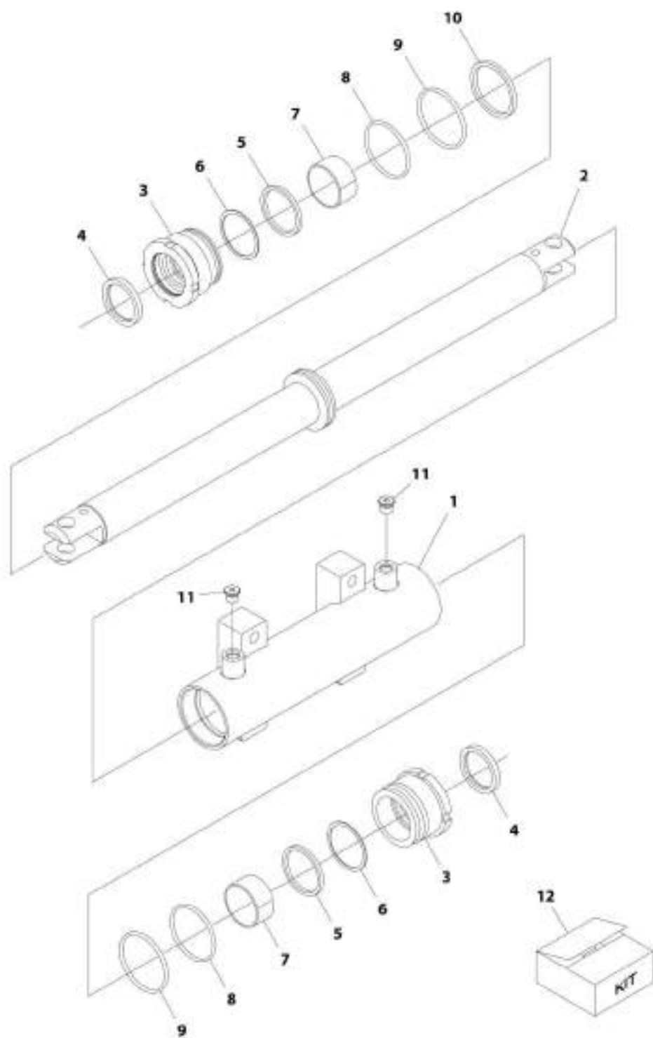
FIGURE 6-11. STEER CYLINDER ASSEMBLY
