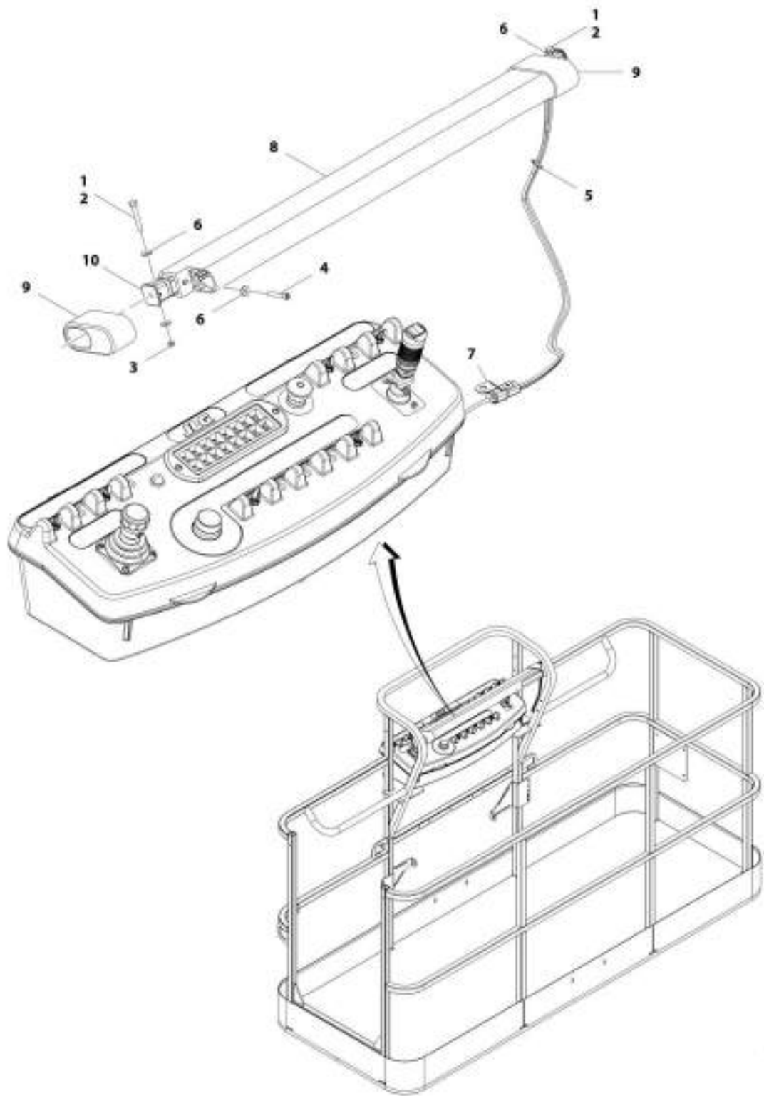
FIGURE 5-31. SKYGUARD SYSTEM INSTALLATION
