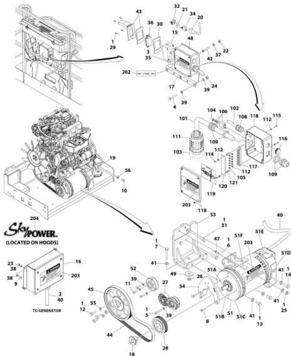
FIGURE 3-70. GENERATOR INSTALLATION - 7500W/60HZ (KUBOTA ENGINE)
