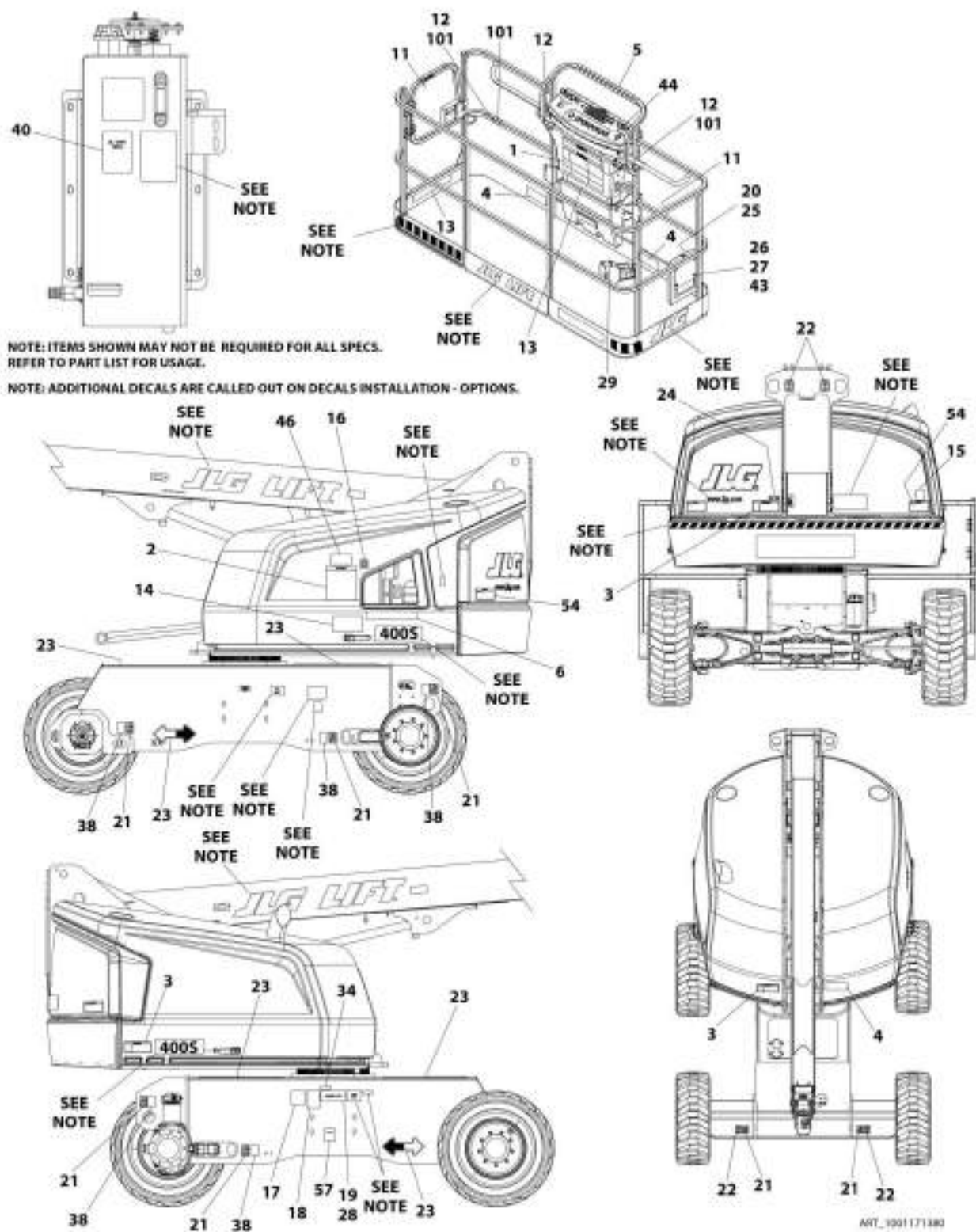
FIGURE 9-8. DECAL INSTALLATION - BRAZIL SPEC (DUAL LANGUAGE - PORTUGUESE/SPANISH) (400S)
