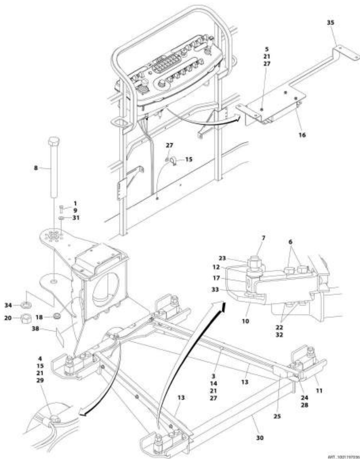
FIGURE 4-17. PLATFORM SUPPORT INSTALLATION WITH 4 CELL LSS
