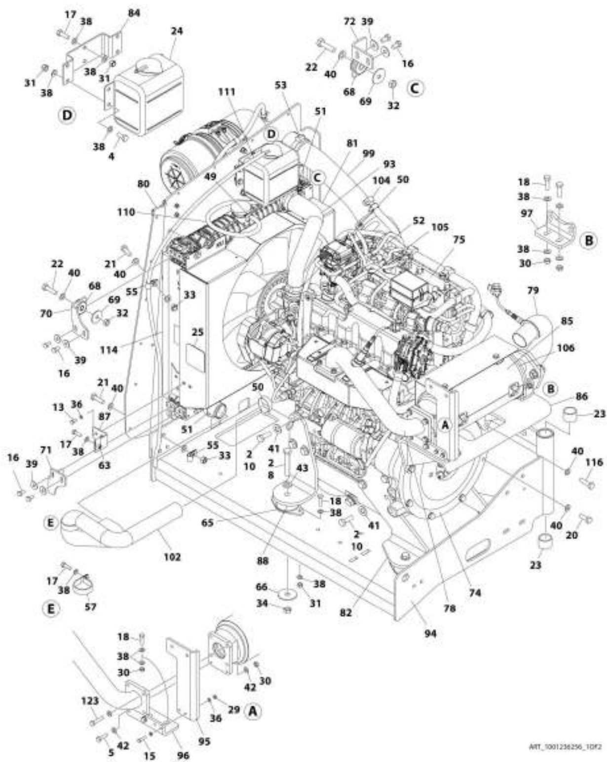
FIGURE 3-39. ENGINE ASSEMBLY - KUBOTA ENGINE (WITHOUT ARCTIC PACKAGE) (SN 0300241778 to Present)
