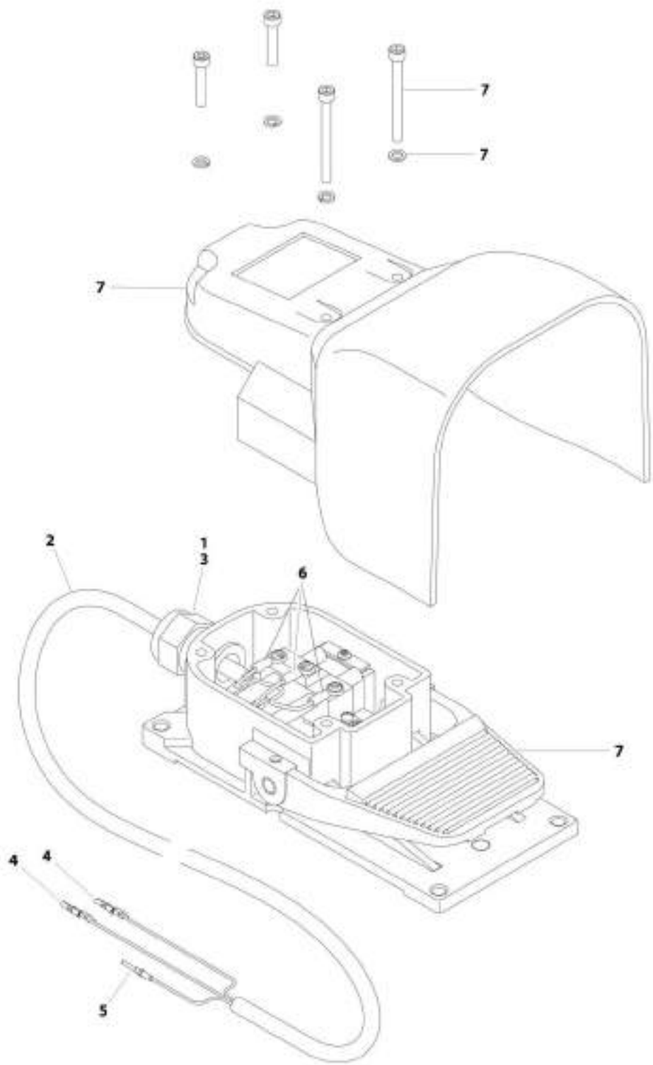
FIGURE 5-25. FOOTSWITCH ASSEMBLY
