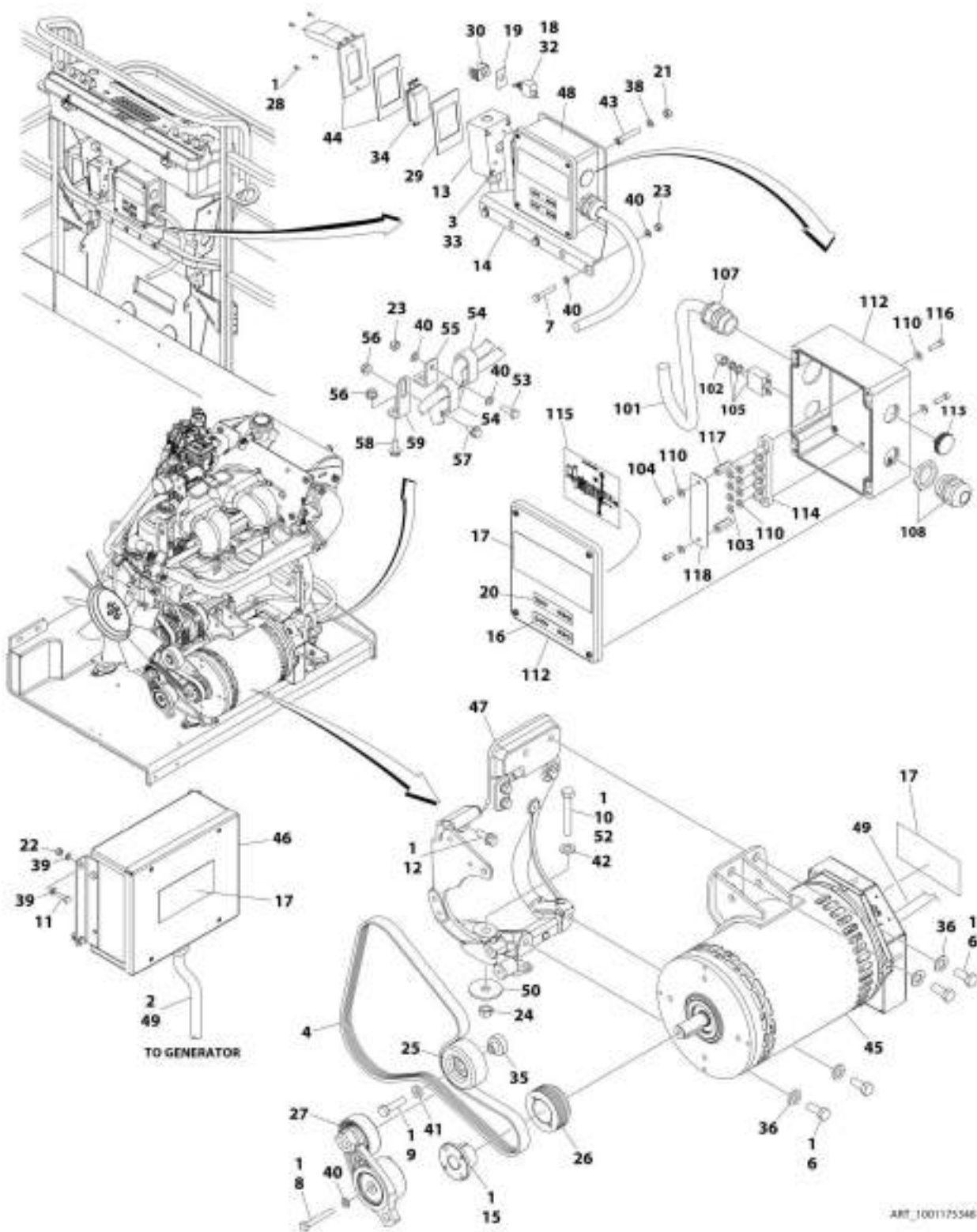
FIGURE 3-65. GENERATOR INSTALLATION - 4000W/60HZ (GM ENGINE)
