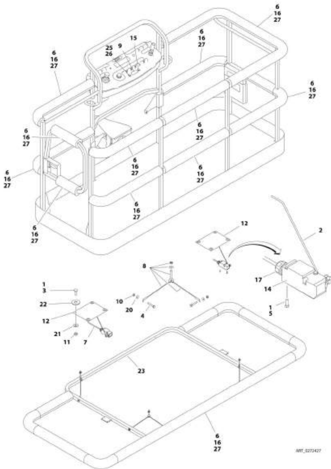
FIGURE 5-30. SOFT TOUCH INSTALLATION - 36IN X 8FT (91.5CM X 2.44M) PLATFORM (OPTIONAL)
