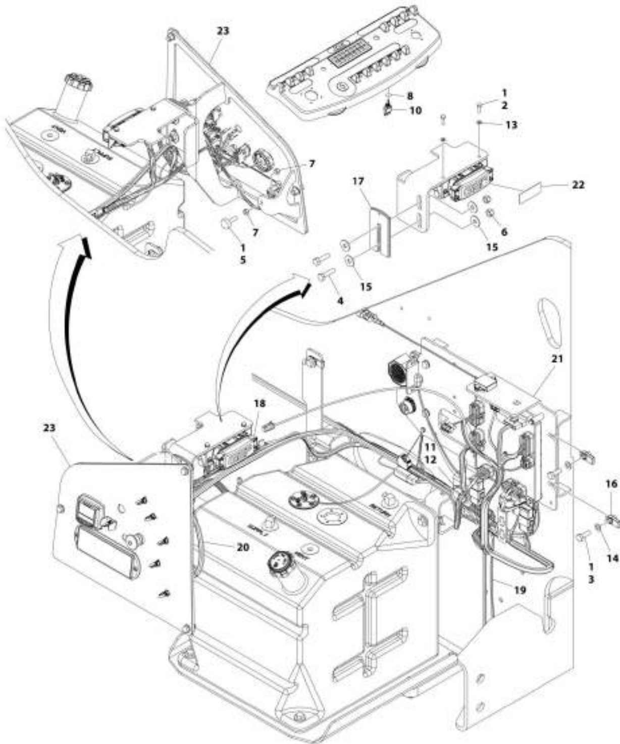
FIGURE 2-23. ELECTRICAL INSTALLATION - 460SJ (ANSI AND CSA SPECS)
