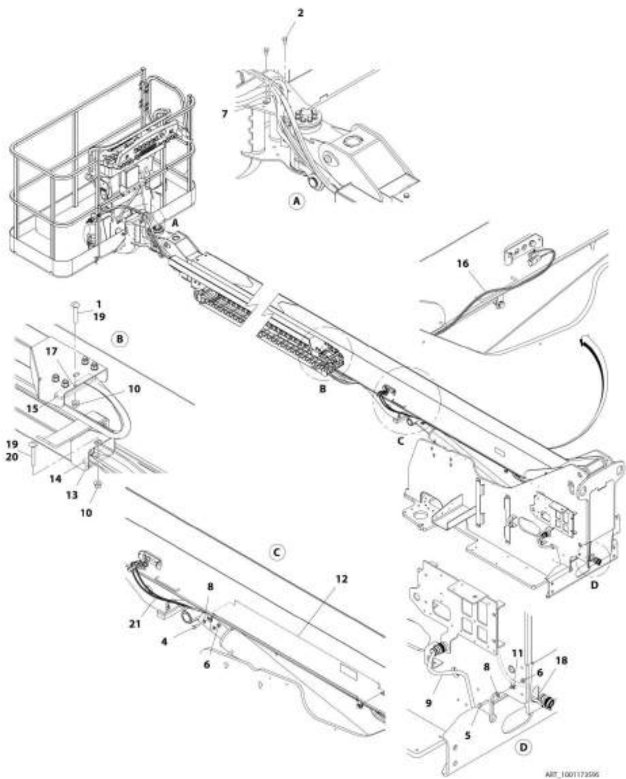
FIGURE 4-20. CABLES AND CLAMPS INSTALLATION - 400S (CE SPECS) (SN 0300203771 through 0300212082)
