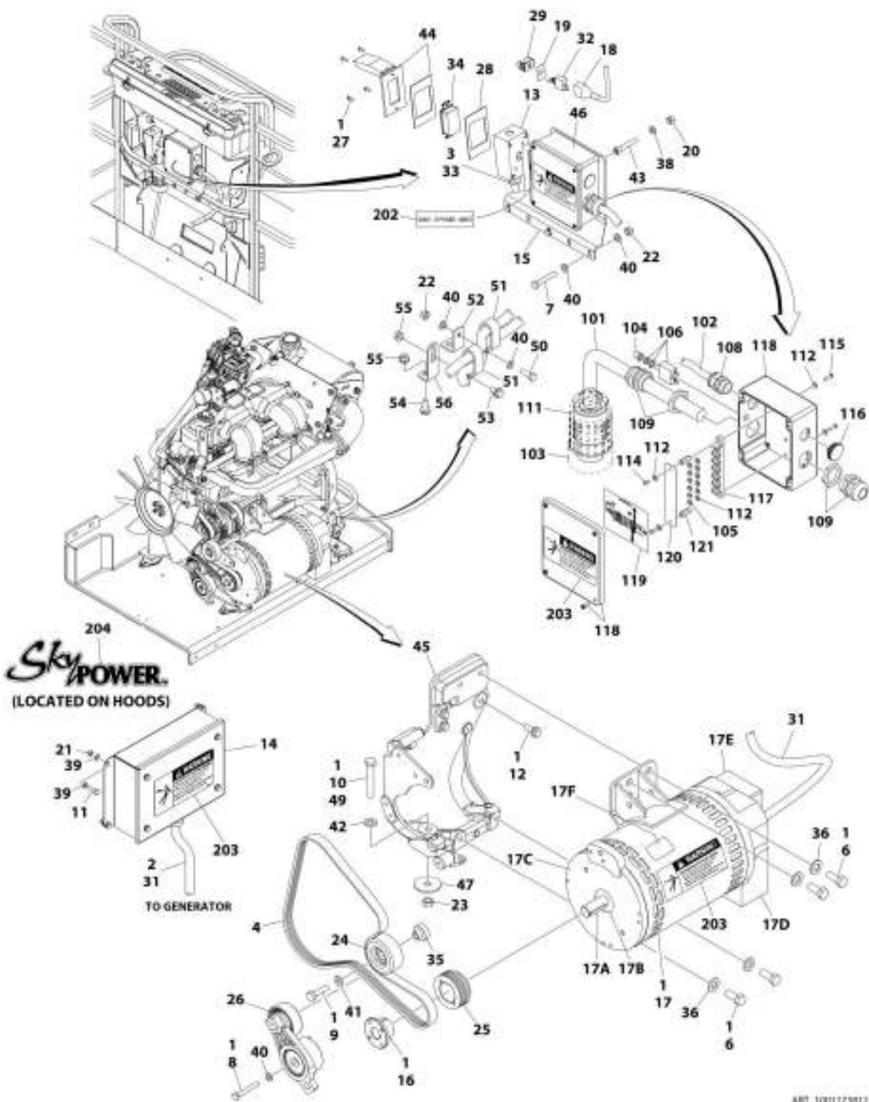
FIGURE 3-69. GENERATOR INSTALLATION - 7500W/60HZ (GM ENGINE)
