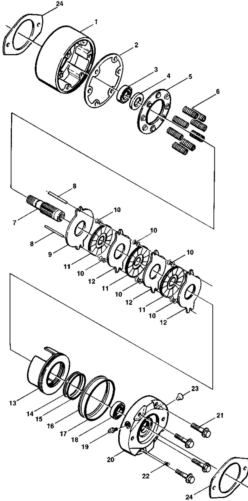
FIGURE 1-3. DRIVE BRAKE ASSEMBLY - AUSCO
