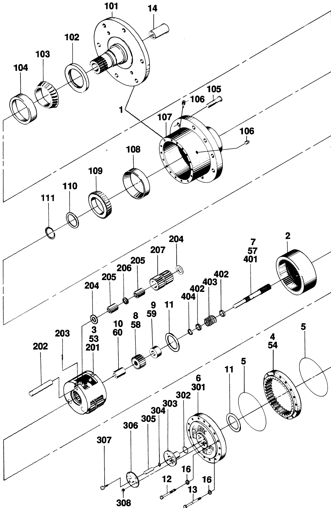
FIGURE 1-6. DRIVE HUB ASSEMBLIES.
