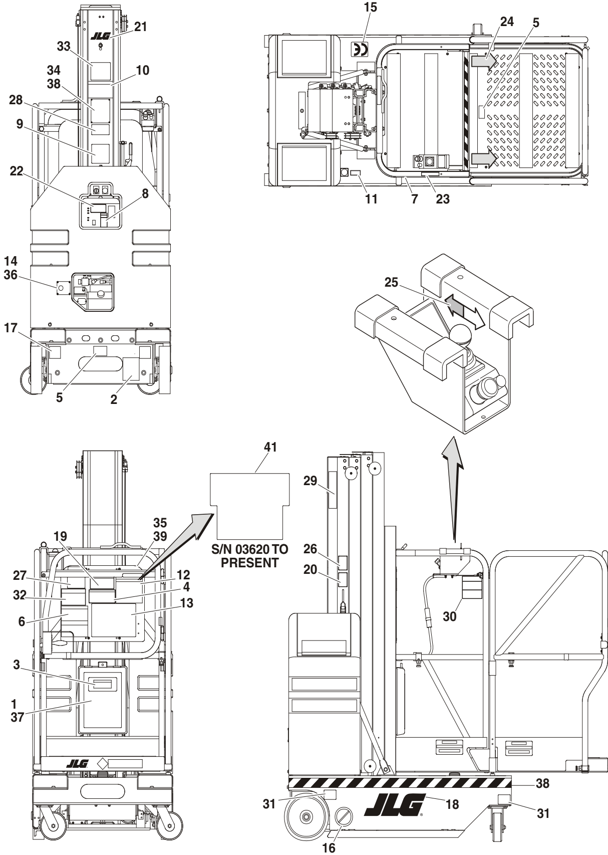
FIGURE 8-1.DECALS INSTALLATION
