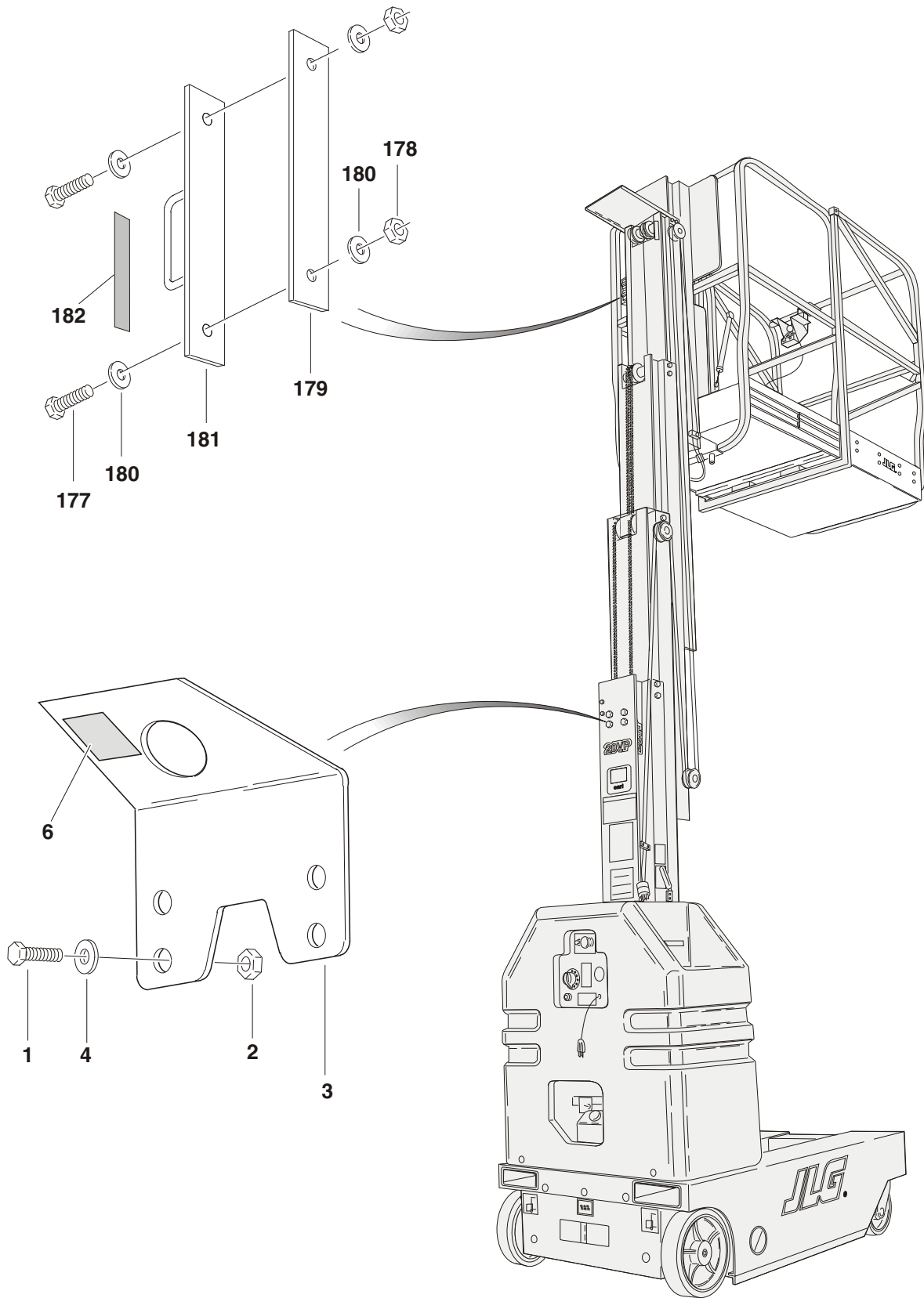
FIGURE 3-2. MAST MOUNTING COMPONENTS
