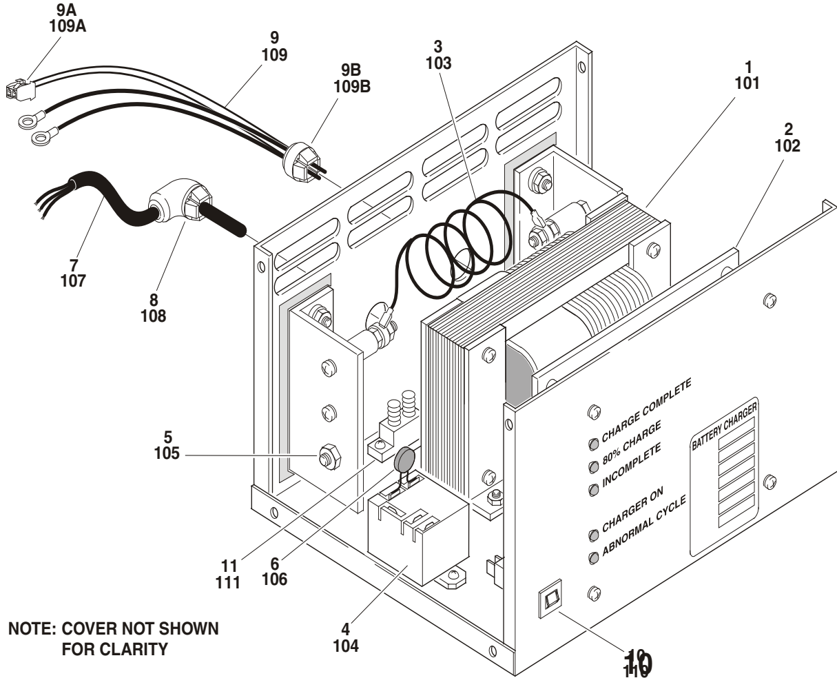
FIGURE 2-3. BATTERY CHARGER ASSEMBLY
