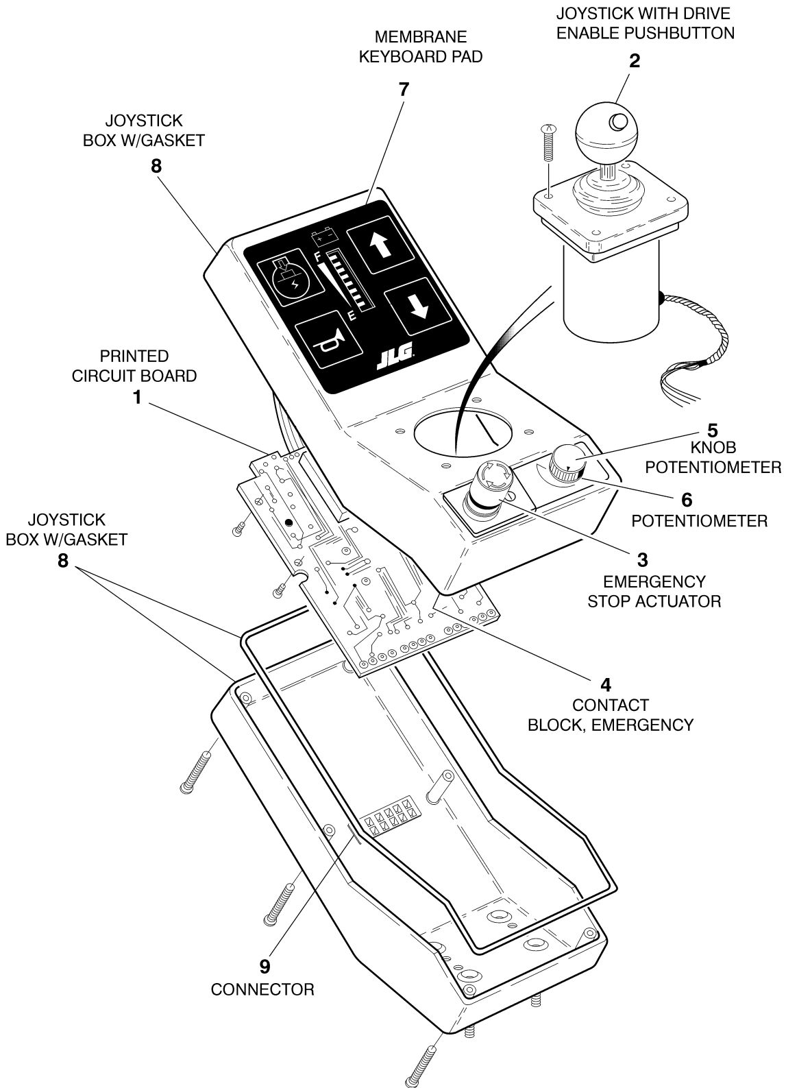
FIGURE 2-5. CONTROL BOX ASSEMBLY
