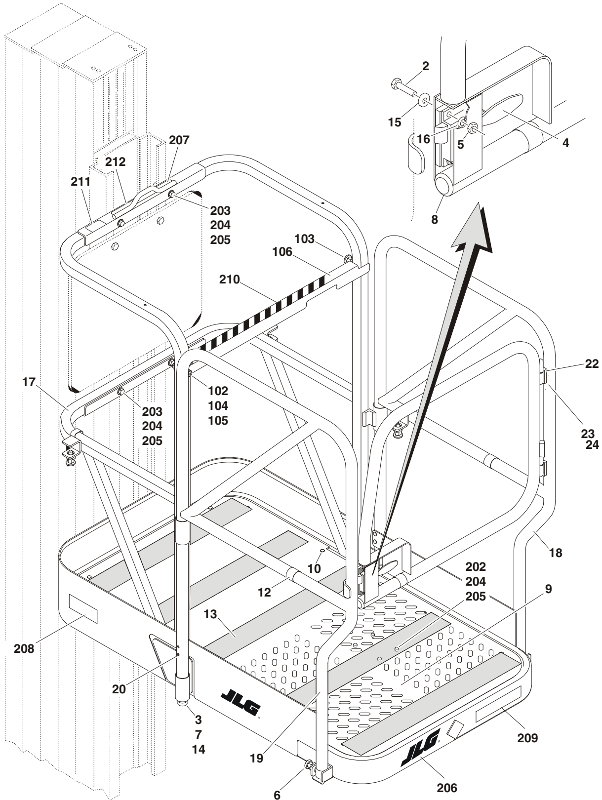
FIGURE 4-2.PLATFORM INSTALLATION (FIXED SIDE RAILS)
