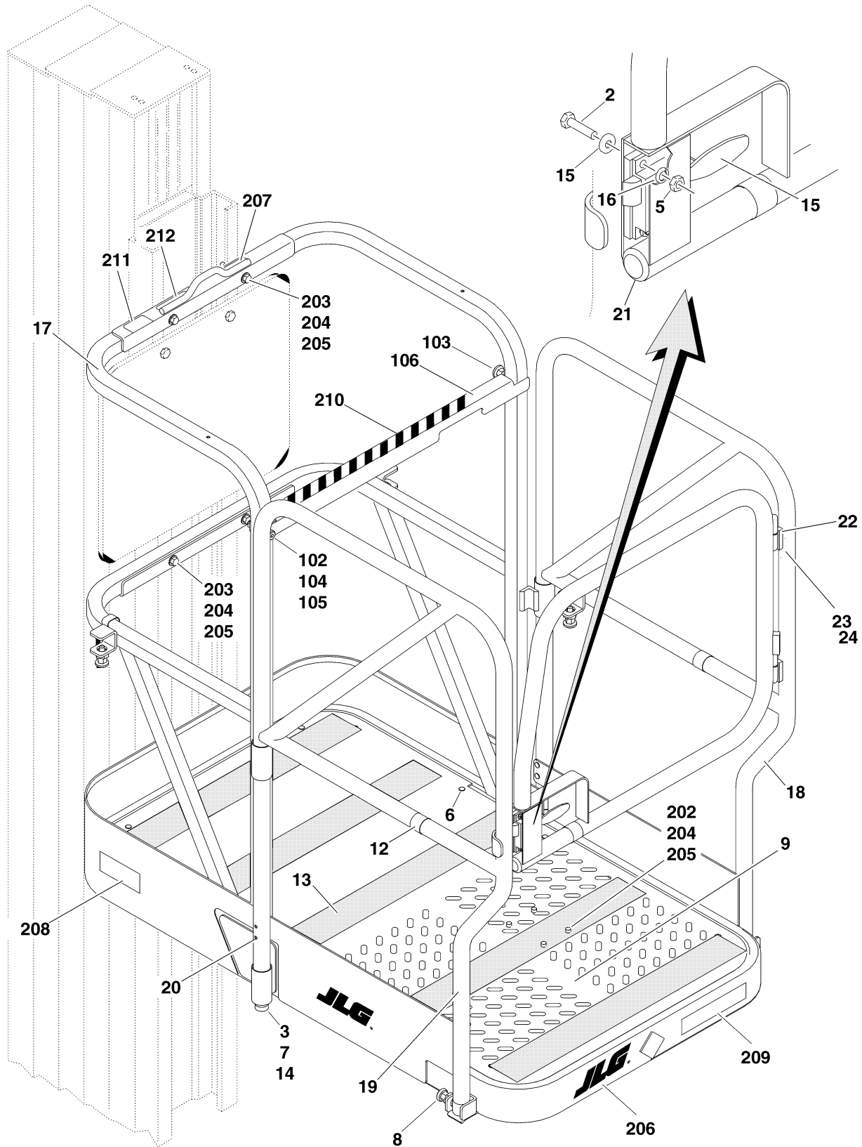
FIGURE 4-1.PLATFORM INSTALLATION (FOLD DOWN SIDE RAILS)
