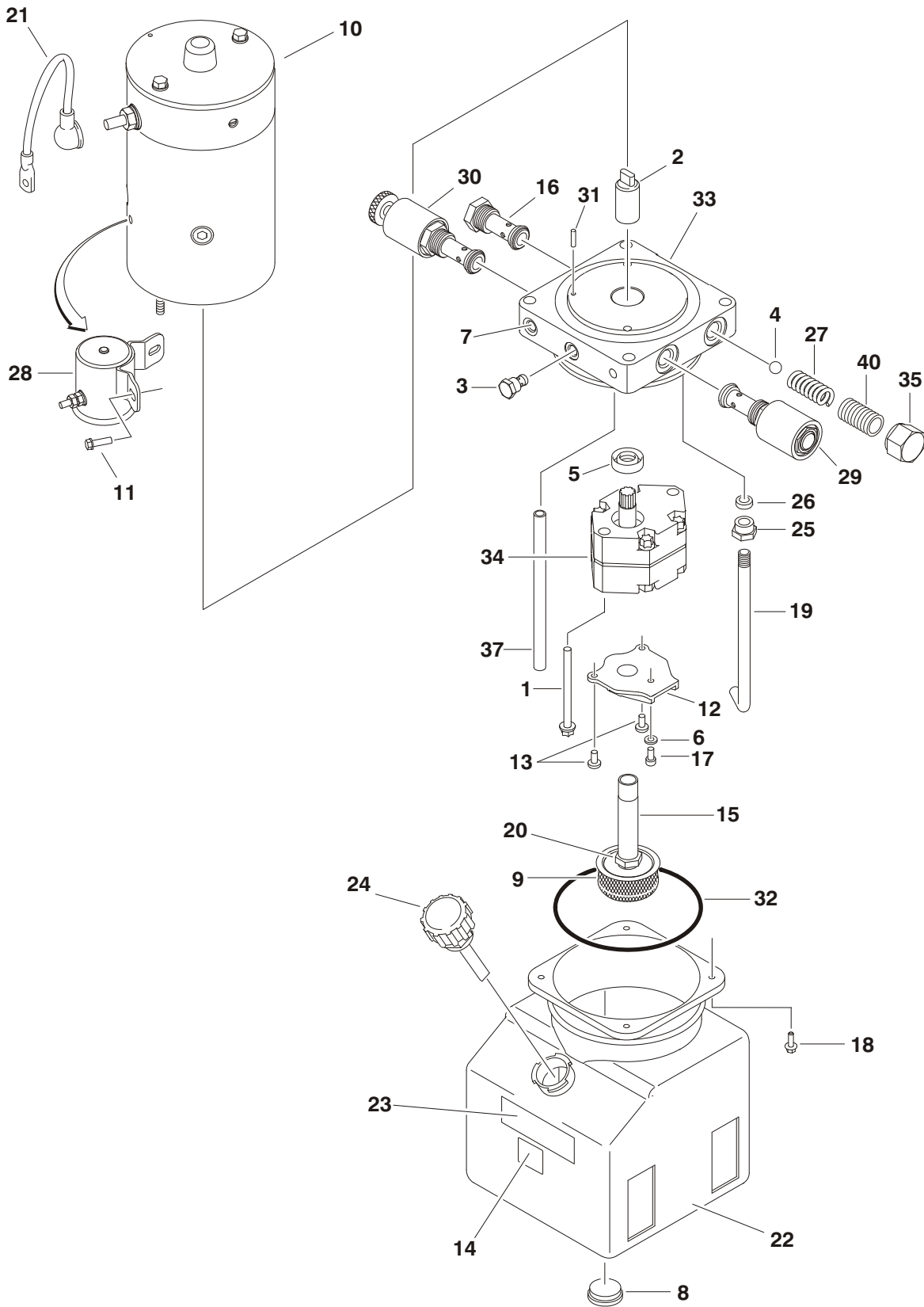
FIGURE 2-4. PUMP/MOTOR/TANK ASSEMBLY
