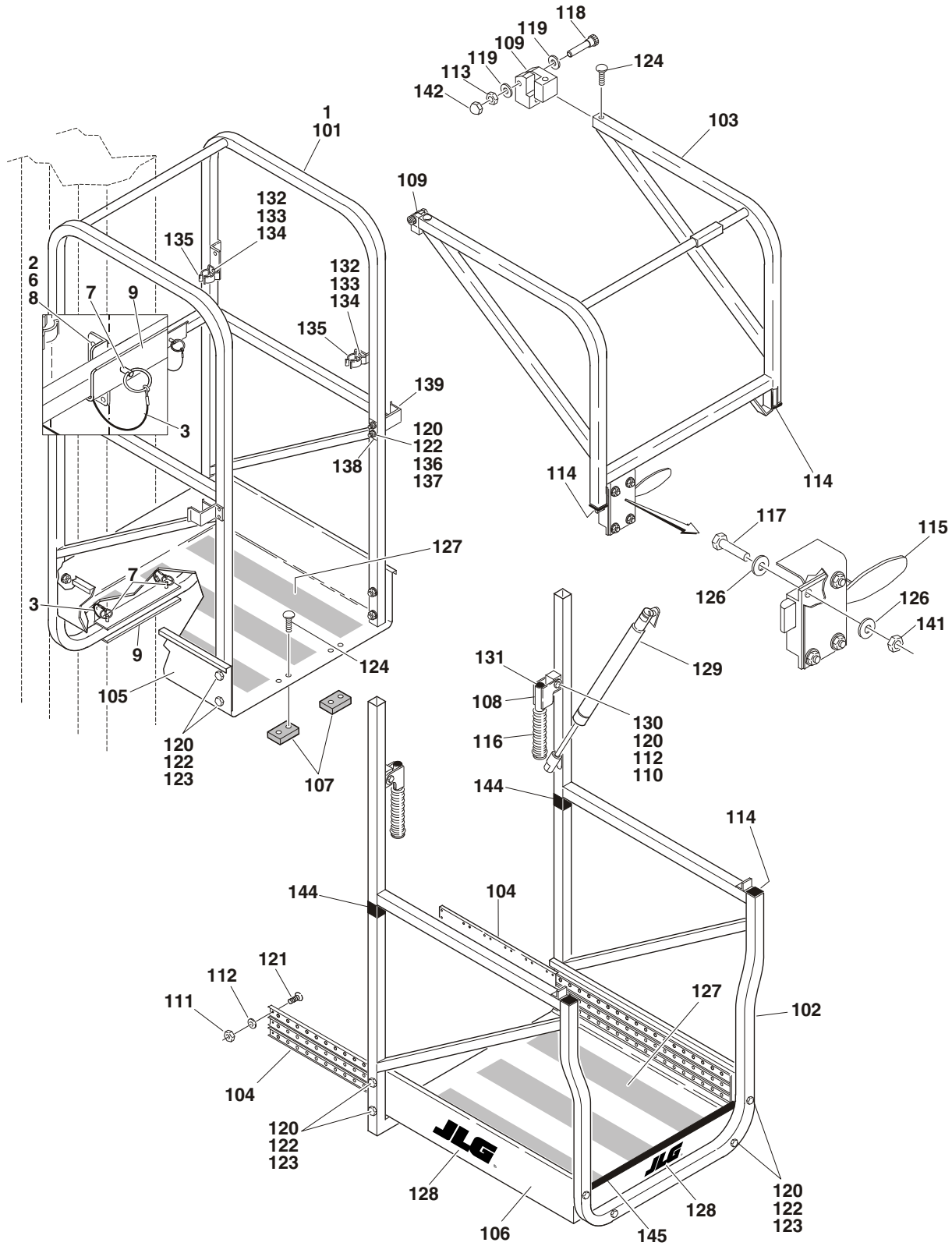
FIGURE 4-3.PLATFORM INSTALLATION (QUICK CHANGE GULLWING)
